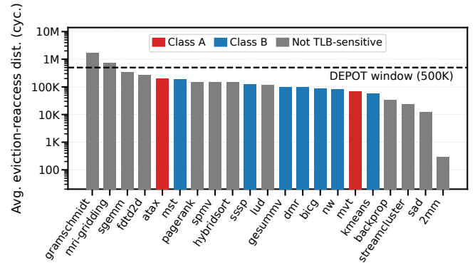
Figure 4: Average eviction-to-reaccess distance (log scale) per workload vs. DEPOT’s default protection window, for all 21 workloads with measurable dead-entry activity.
