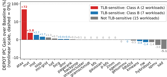
Figure 7: IPC improvement of DEPOT over 4 KB baseline for all 24 workloads, sorted descending.
