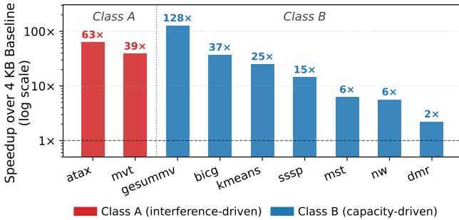
Figure 5: IPC speedup under 2 MB pages over 4 KB baseline for all 9 TLB-sensitive workloads.
