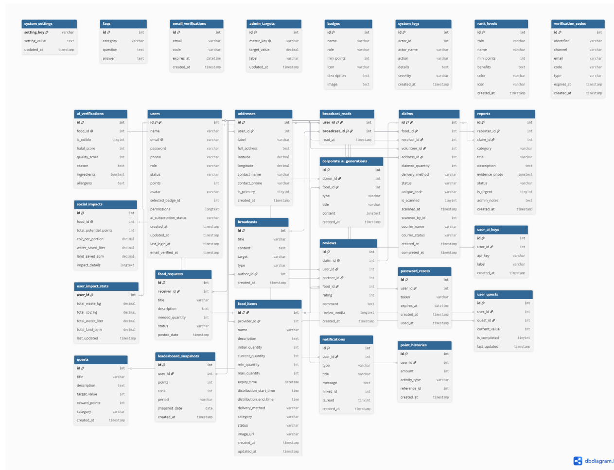
Gambar 3.2: Entity Relationship Diagram (ERD) Food AI Rescue
