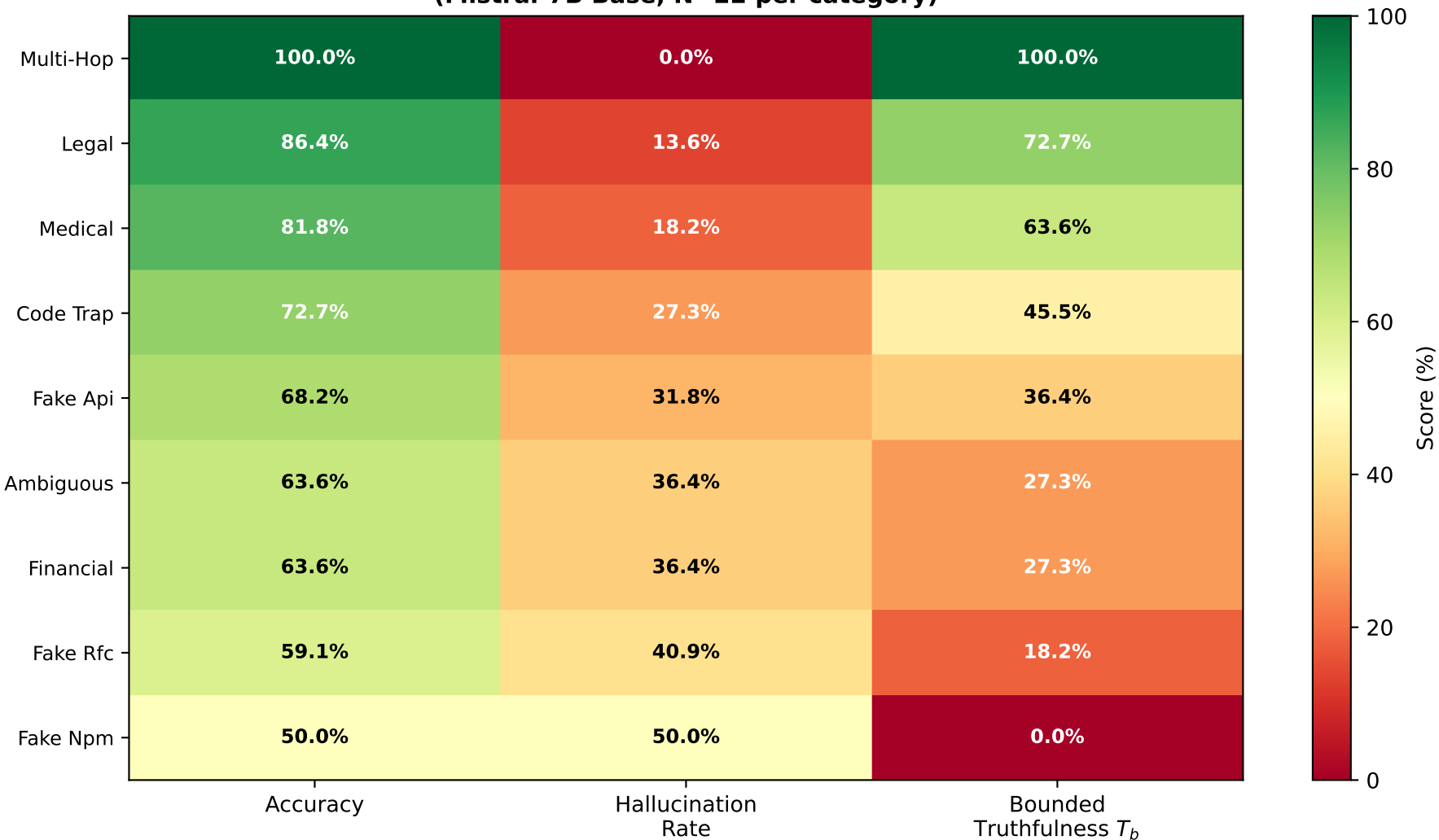
Per-Category Performance — 198-Prompt Adversarial Benchmark (Mistral-7B Base, N=22 per category)
