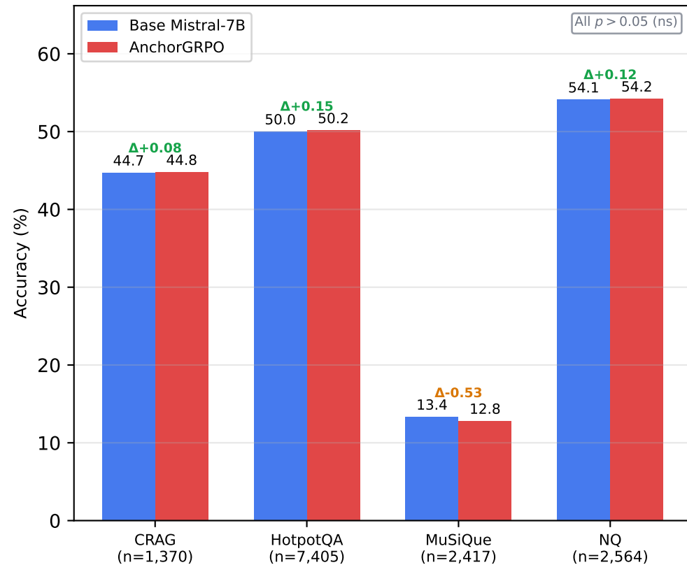
Accuracy
