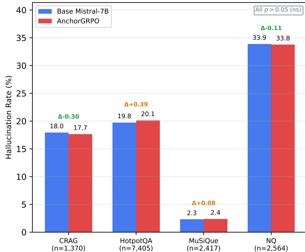
Hallucination Rate
