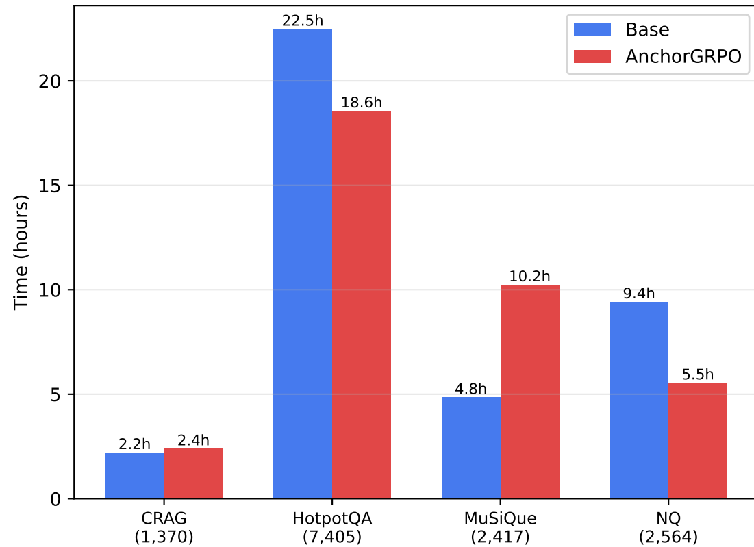
Absolute Inference Time
