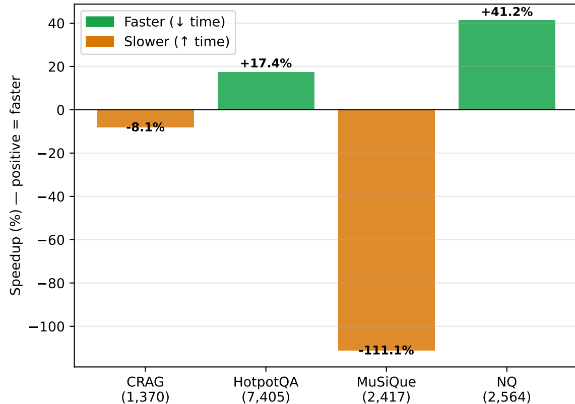
Relative Speedup (AnchorGRPO vs. Base)
