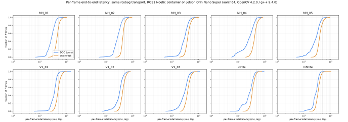
Fig. 3. Per-frame latency CDFs on the Orin Nano Super, both estimators, all ten sequences (log scale; dotted line: the 50 ms EuRoC 20 Hz frame budget). Direction matches x86 (Figure 2); the margin does not.
