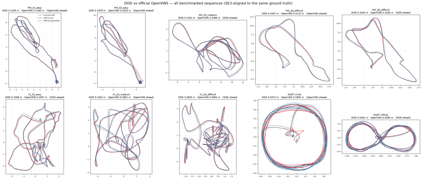
Fig. 1. Estimated trajectories for all ten benchmarked sequences, both estimators SE(3)-aligned to the same ground truth by the same Uneyama fit used to score Table II (Uneyama alignment removes the initialization-timing offset that Section V-F discusses, so this figure is a shape/consistency check, not a re-derivation of the ATE numbers). KAIST circle’s red (ours) trace visibly loops near the origin before settling onto the ground-truth circle – the initialization-latency transient discussed in Section VII.
