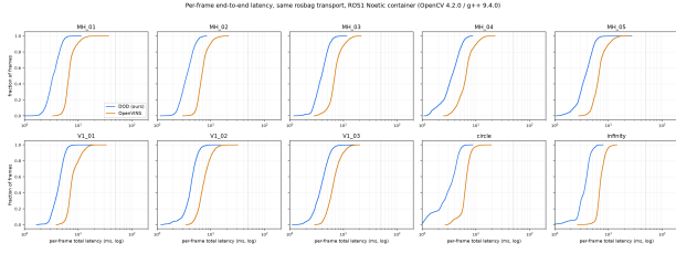
Fig. 1. Per-frame latency CDFs on x86, both estimators, all ten sequences (log scale; dotted line: the 50 ms EuRoC 20 Hz frame budget).
