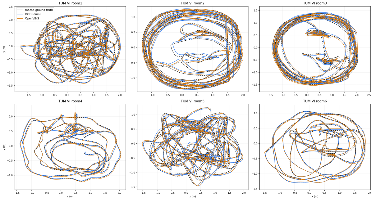
Fig. 3. TUM VI room1–6: both estimators Umeyama-aligned to the mocap ground truth. All twelve runs (six per estimator) initialize and converge; no sequence was tuned for.
