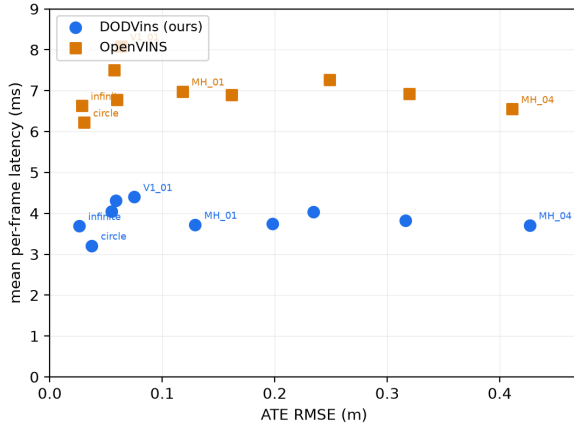
Fig. 2. The accuracy/efficiency trade-off per sequence, x86: mean per-frame latency (y) against ATE (x). DODVins’s points sit below OpenVINS’s on every sequence at statistically equal accuracy — the speedup does not purchase accuracy anywhere on the benchmark.
