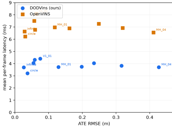
Fig. 2. The accuracy/efficiency trade-off per sequence, x86: mean per-frame latency (y) against ATE (x). DODVins’s points sit below OpenVINS’s on every sequence at statistically equal accuracy; the speedup does not purchase accuracy anywhere on the benchmark.
