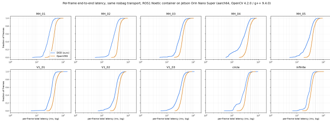
Fig. 4. Per-frame latency CDFs on the Orin Nano Super, both estimators, all ten sequences (log scale; dotted line: the 50 ms EuRoC 20 Hz frame budget). Direction matches x86 (Figure 2); the margin does not.
