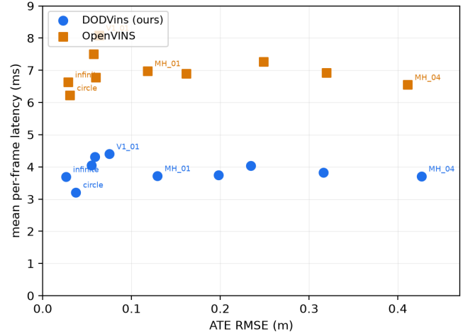
Fig. 3. The accuracy/efficiency trade-off per sequence, x86: mean per-frame latency (y) against ATE (x). DODVins’s points sit below OpenVINS’s on every sequence at statistically equal accuracy — the speedup does not purchase accuracy anywhere on the benchmark.
