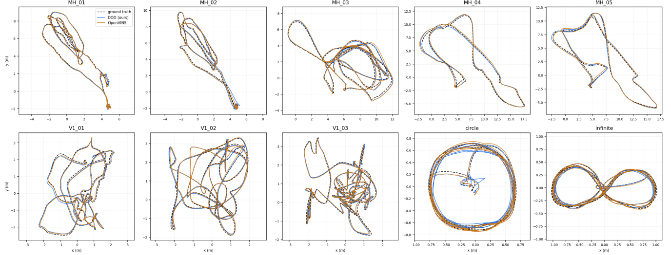
Fig. 1. Estimated trajectories for all ten benchmarked sequences, both estimators SE(3)-aligned to the same ground truth by the same Umeyama fit used to score Table II (Umeyama alignment removes the initialization-timing offset that Section V-F discusses, so this figure is a shape/consistency check, not a re-derivation of the ATE numbers). Regenerated from the same fresh 2026-08-30 runs as Table II. KAIST circle’s blue (ours) trace visibly loops near the origin before settling onto the ground-truth circle – the initialization-latency transient discussed in Section VIII.
