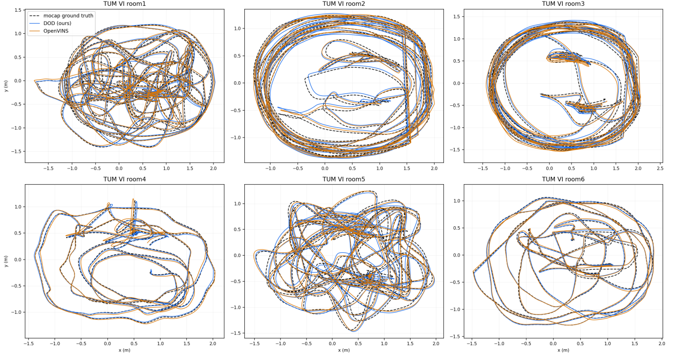
Fig. 5. TUM VI room1–6: both estimators Umeyama-aligned to the mocap ground truth. All twelve runs (six per estimator) initialize and converge; no sequence was tuned for.
