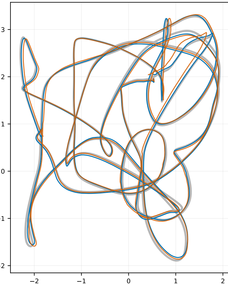
V1_02_medium DOD 0.0589 m OpenVINS 0.0573 m (OpenVINS ahead)
