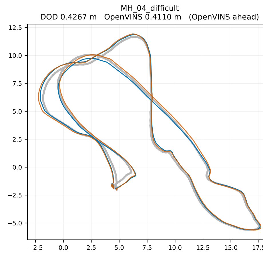
MH_04_difficult DOD 0.4267 m OpenVINS 0.4110 m (OpenVINS ahead)
