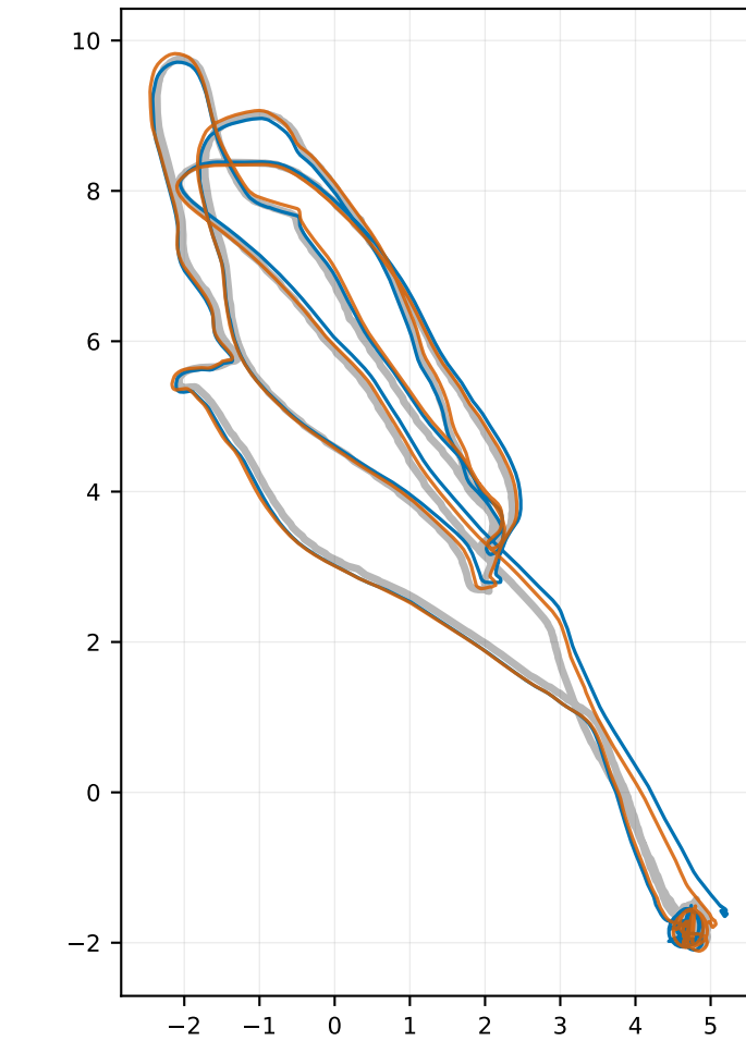
V1_02_medium DOD 0.0589 m OpenVINS 0.0573 m (OpenVINS ahead)
