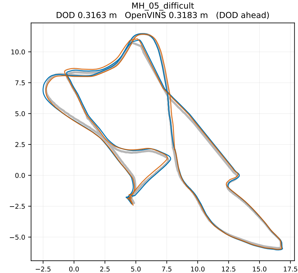
MH_05_difficult DOD 0.3163 m OpenVINS 0.3183 m (DOD ahead)
