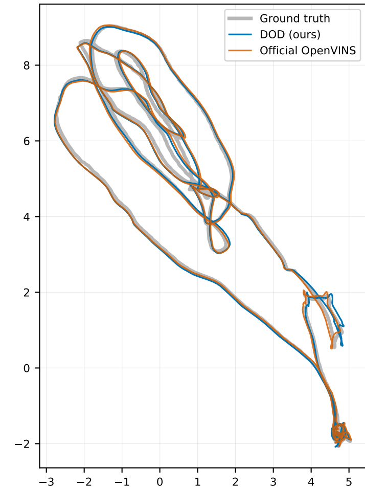
V1_01_easy DOD 0.0751 m OpenVINS 0.0634 m (OpenVINS ahead)
