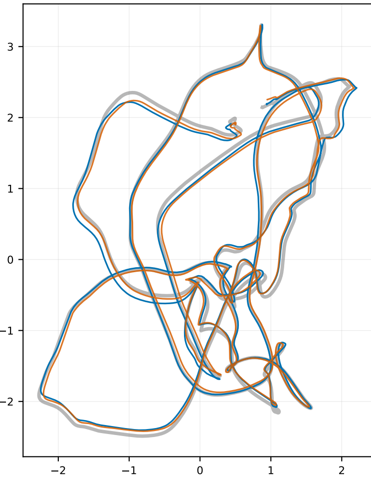
V1_01_easy DOD 0.0751 m OpenVINS 0.0634 m (OpenVINS ahead)
