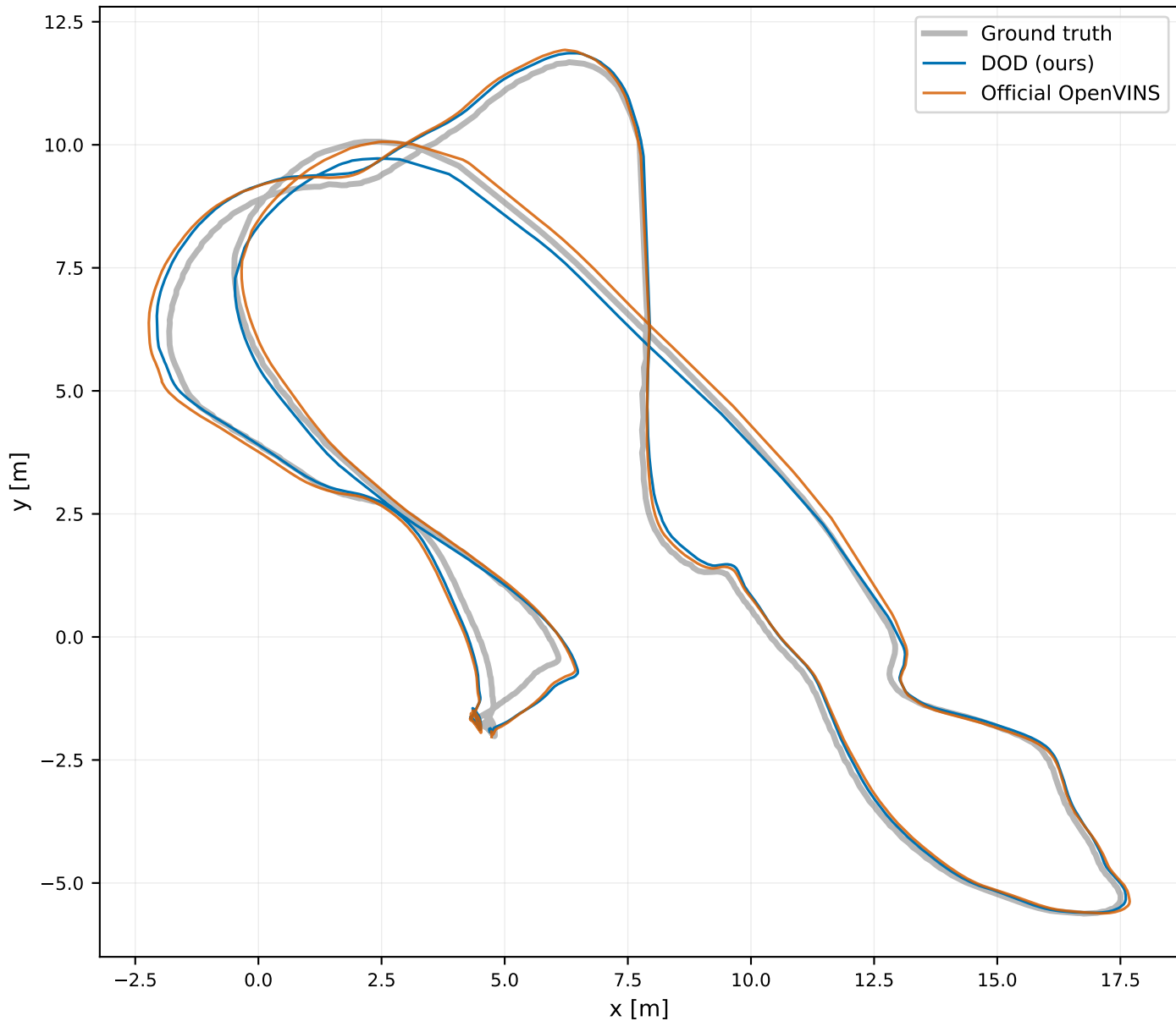
MH_04_difficult DOD 0.4267 m OpenVINS 0.4110 m (OpenVINS ahead)
