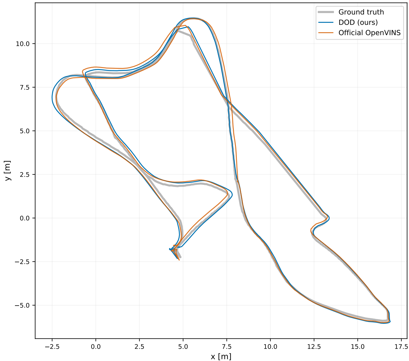
MH_05_difficult DOD 0.3163 m OpenVINS 0.3183 m (DOD ahead)
