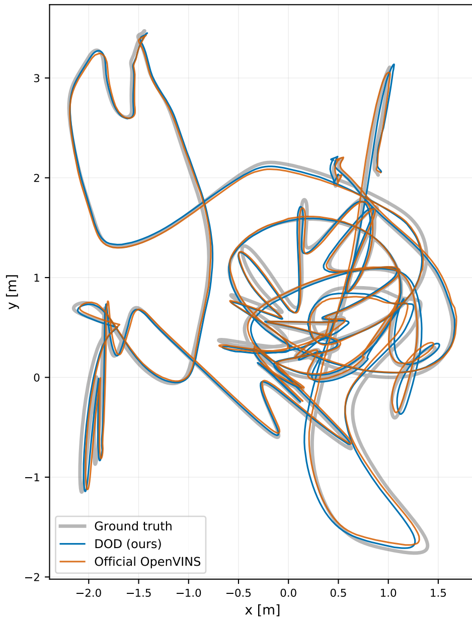
V1_03_difficult DOD 0.0550 m OpenVINS 0.0595 m (DOD ahead)
