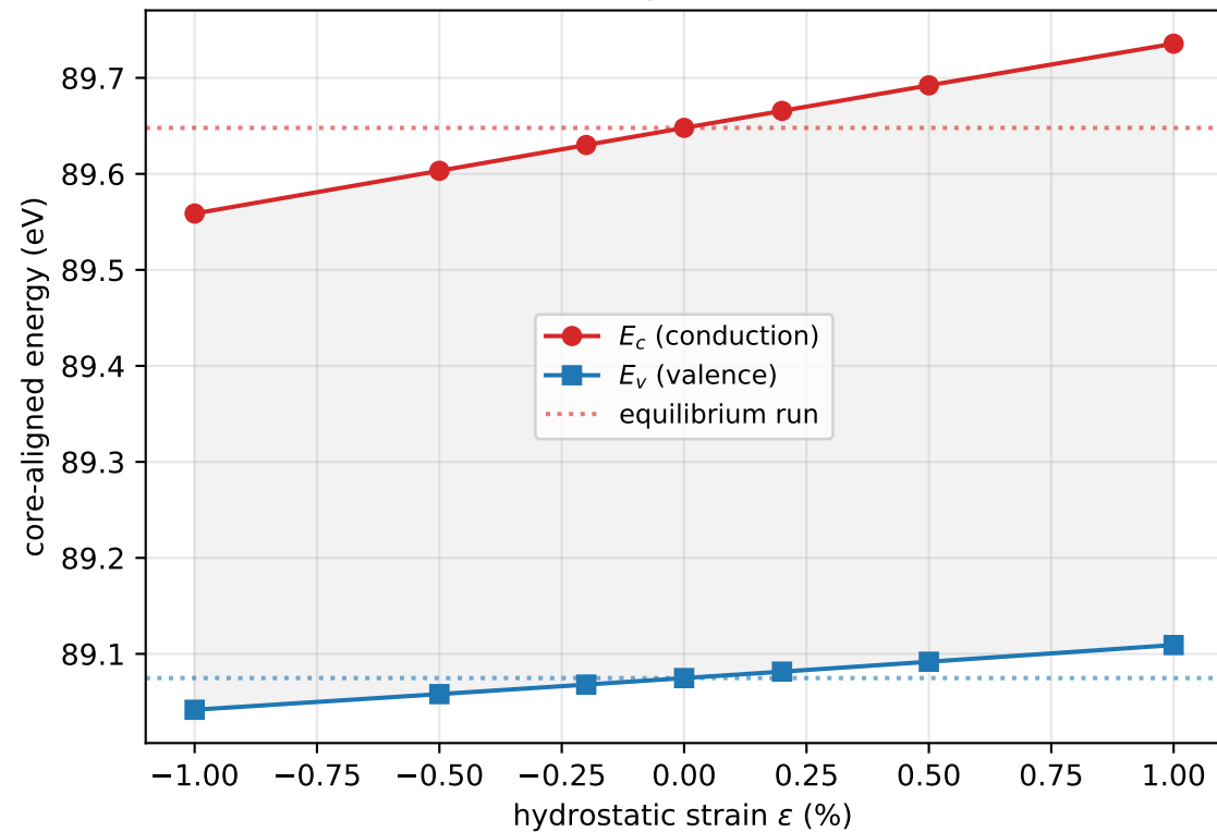
Band edges vs. strain
