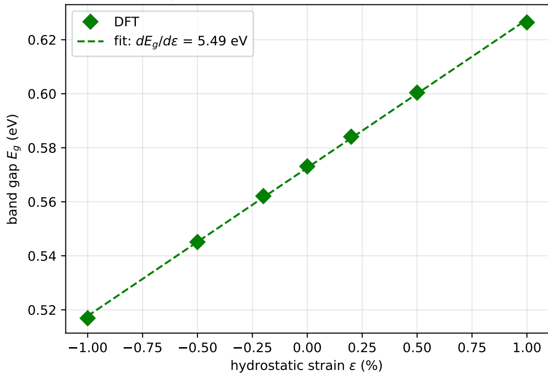
Gap vs. strain (RMS residual 0.62 meV)
