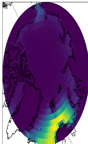
EC-AEREarth3 - Arctic - DMS Emissions (2xDMS)
