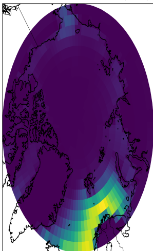
EC-AEREarth3 - Arctic - DMS Emissions (control)
