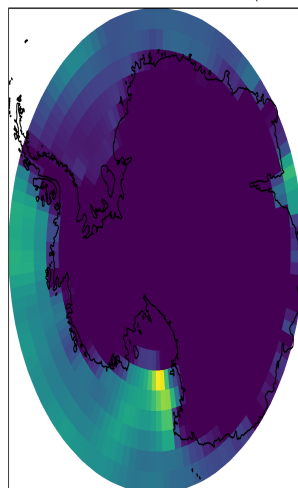
EC-AEREarth3 - Antarctic - DMS Emissions (2xDMS)
