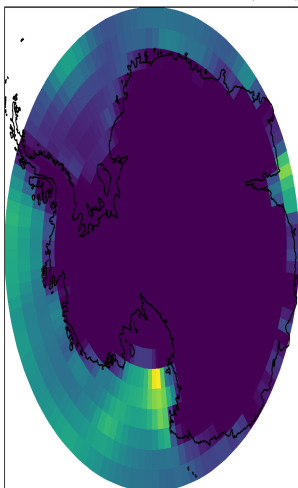
EC-AEREarth3 - Antarctic - DMS Emissions (control)
