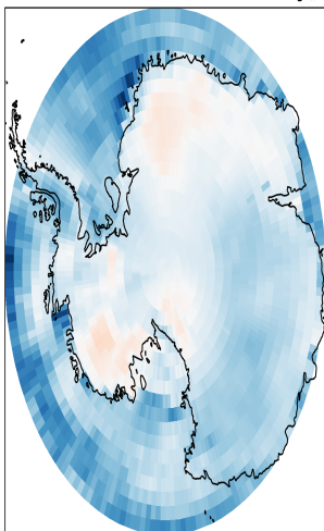
UKESM - Antarctic - Effective Radiative Forcing (I)
