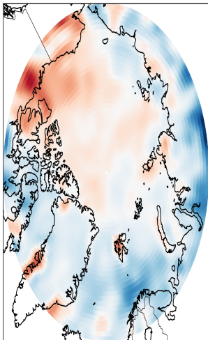
EC-AEREarth3 - Arctic - Effective Radiative Forcing (I)
