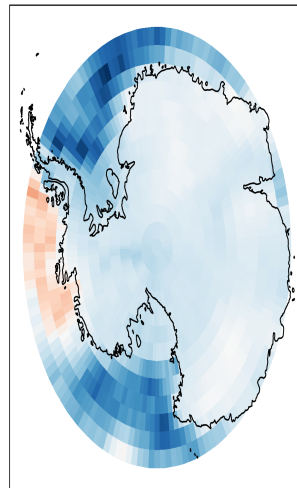
NorESM - Antarctic - Effective Radiative Forcing (I)
