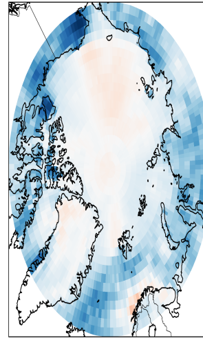
UKESM - Arctic - Effective Radiative Forcing (l)
