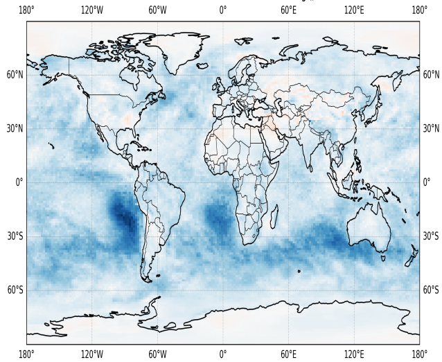
UKESM - Global - Effective Radiative Forcing (l)
