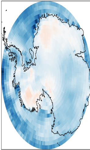
UKESM - Antarctic - Effective Radiative Forcing (l)
