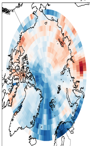
NorESM - Arctic - Effective Radiative Forcing (I)
