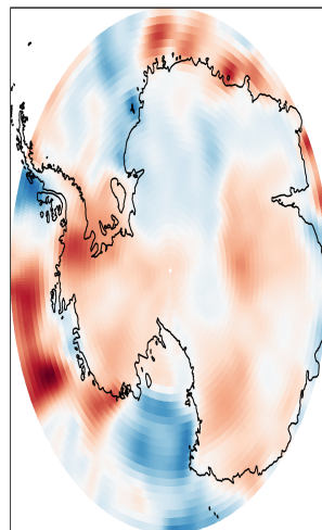
EC-AEREarth3 - Antarctic - Effective Radiative Forcing (I)
