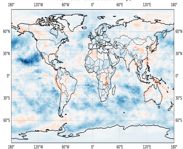
NorESM - Global - Effective Radiative Forcing (I)
