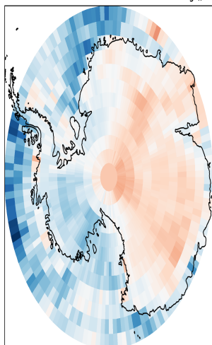
GISS - Antarctic - Effective Radiative Forcing (I)
