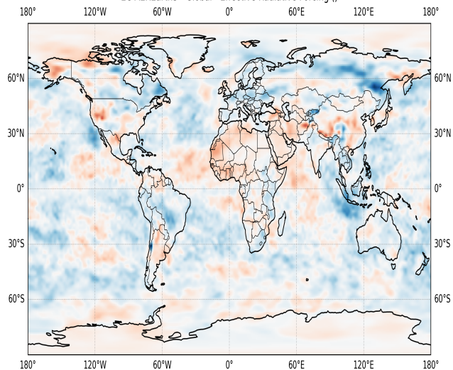
EC-AEREarth3 - Global - Effective Radiative Forcing (I)
