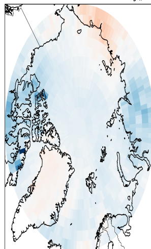
GISS - Arctic - Effective Radiative Forcing (I)
