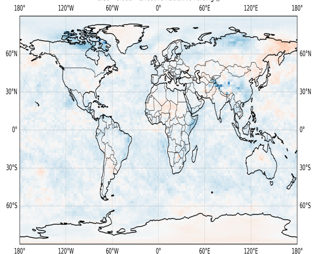
GISS - Global - Effective Radiative Forcing (I)
