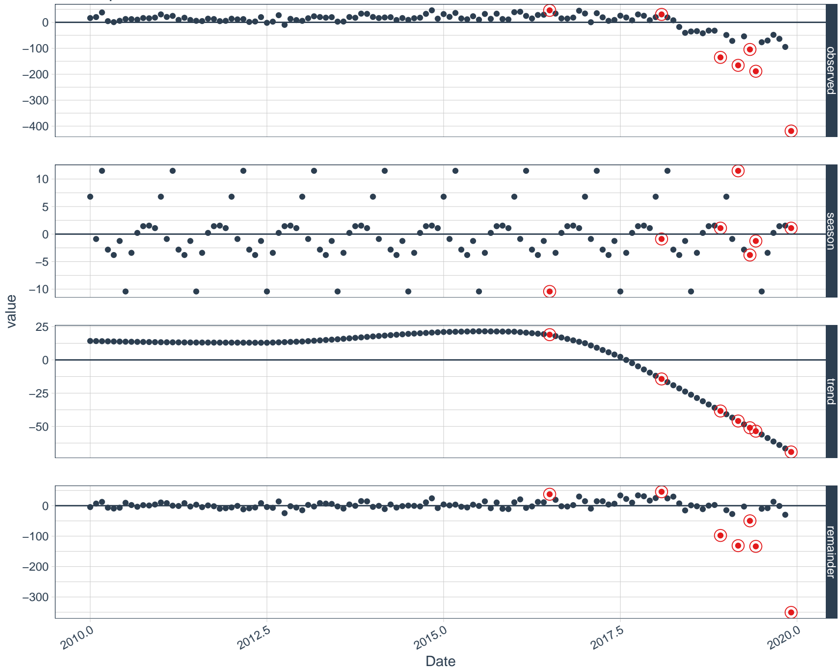
Decomposition of Anomalized PBT data for: Business A
