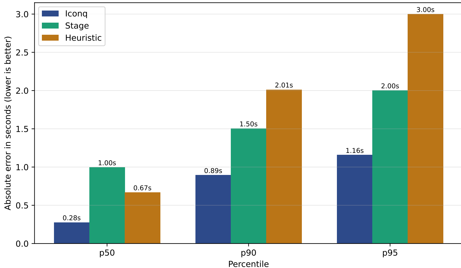
Experiment 1 — Predictor Absolute Error
