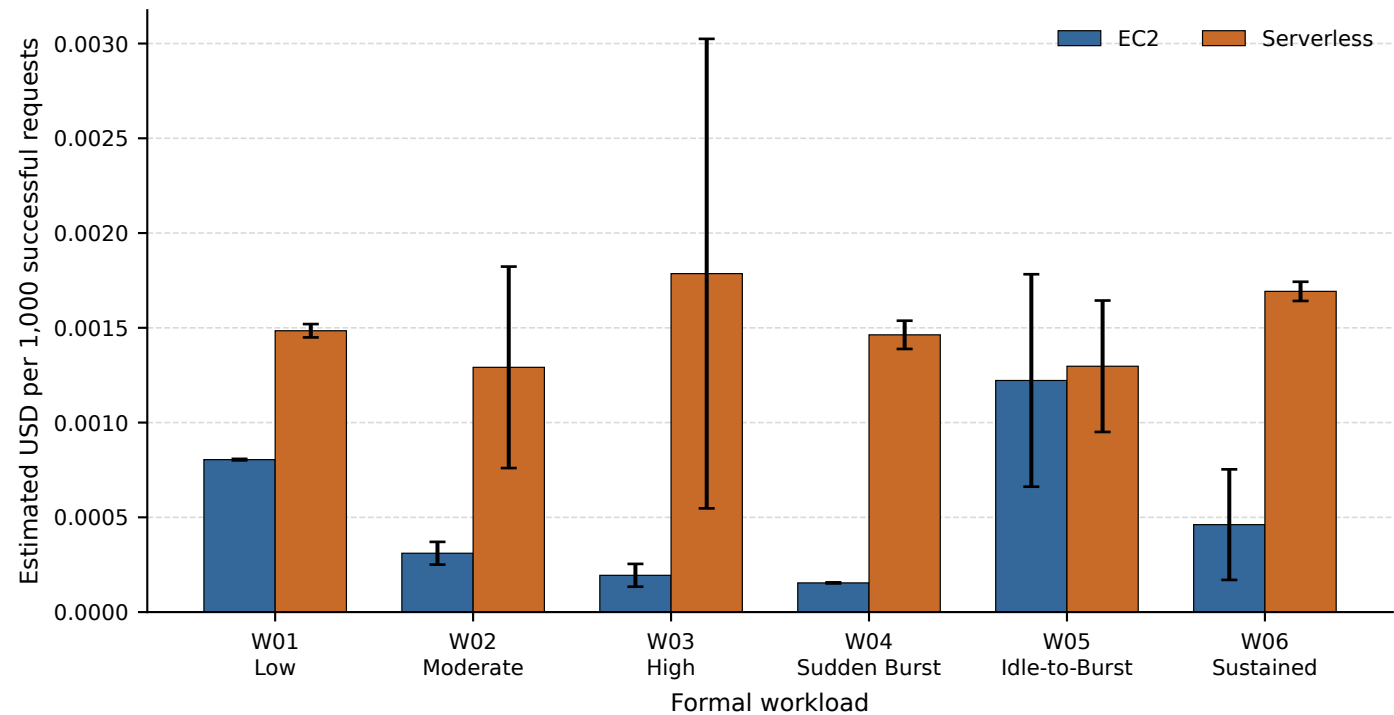
Estimated Cost Efficiency by Workload
