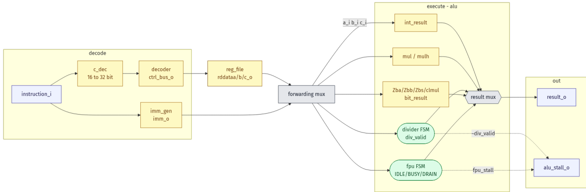
Figure 10: Decode and execute datapath. The instruction word enters on the left, is expanded (if compressed) and decoded into ctrl_bus_o plus an immediate, operands are read and forwarded, and the ALU produces result_o . Only the two FSM blocks (green)—the divider and the FPU—can raise alu_stall_o .
