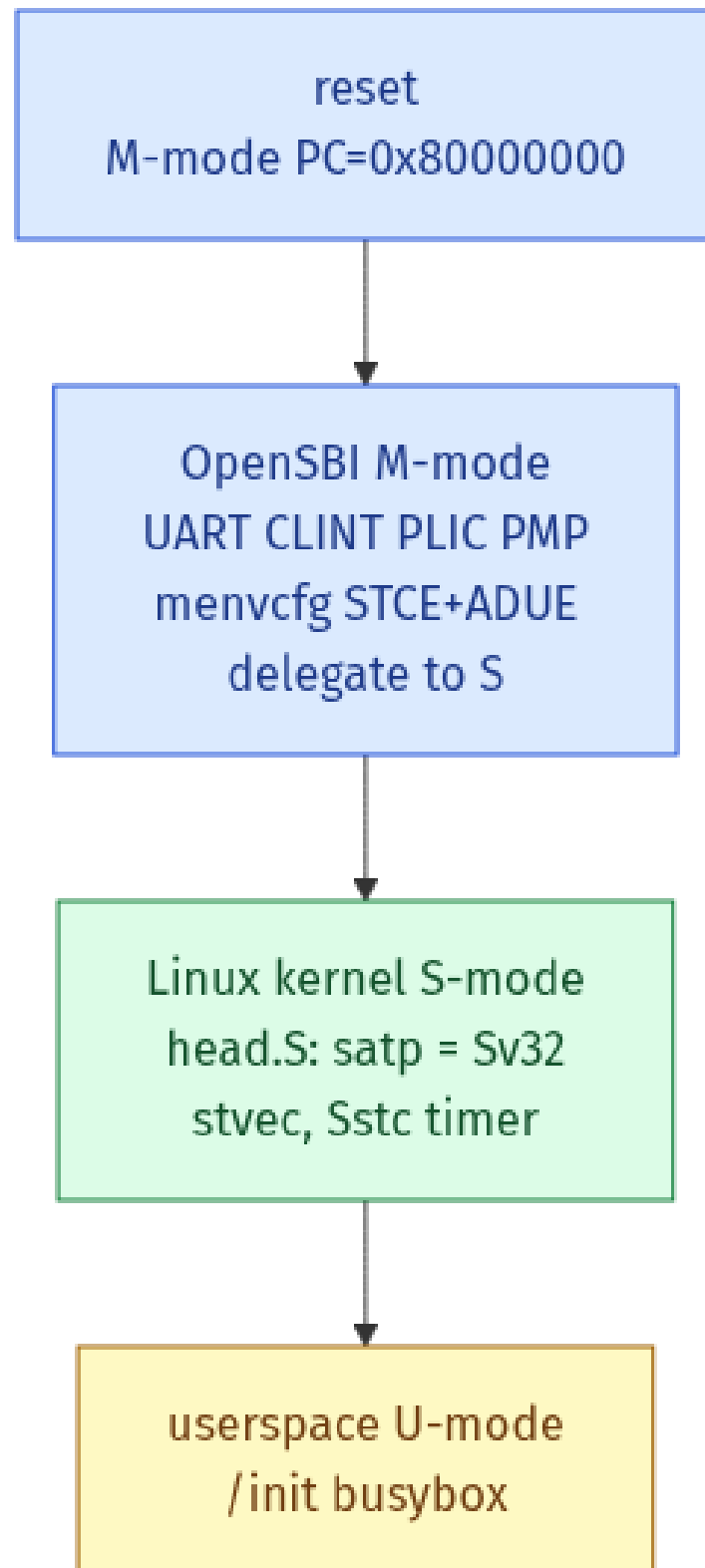
Figure 11: The four boot phases. Privilege drops from M to S to U. Each box lists the main work of that phase.
