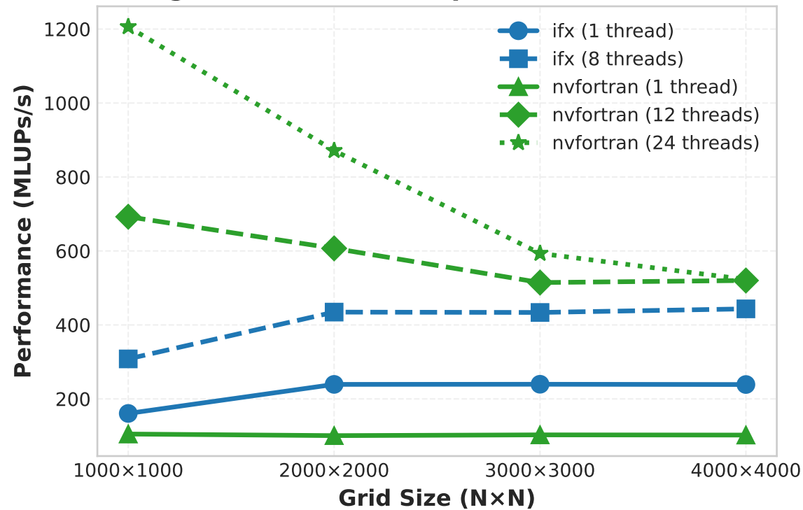
(c) Single Precision - Computational Performance
