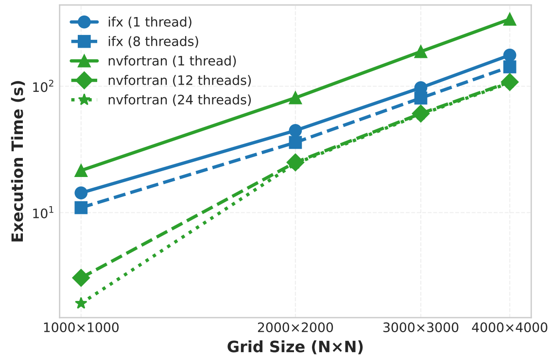
(b) Double Precision - Execution Time
