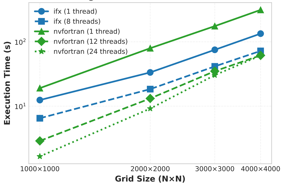
(a) Single Precision - Execution Time
