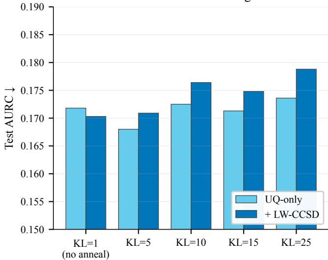
EDL AURC across KL annealing schedules
