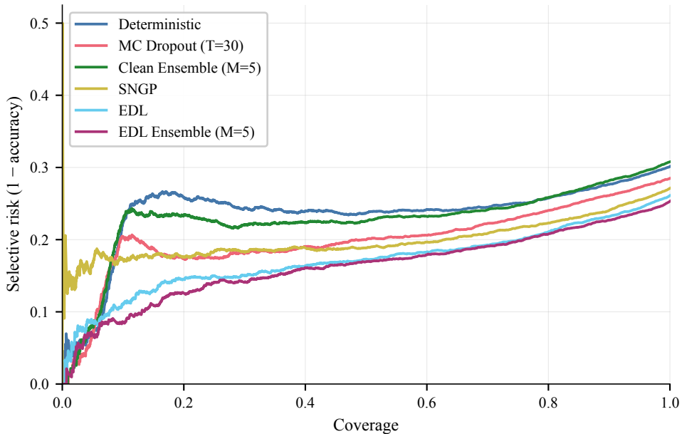
Risk–coverage curves (CinC test, n=6,750 )
