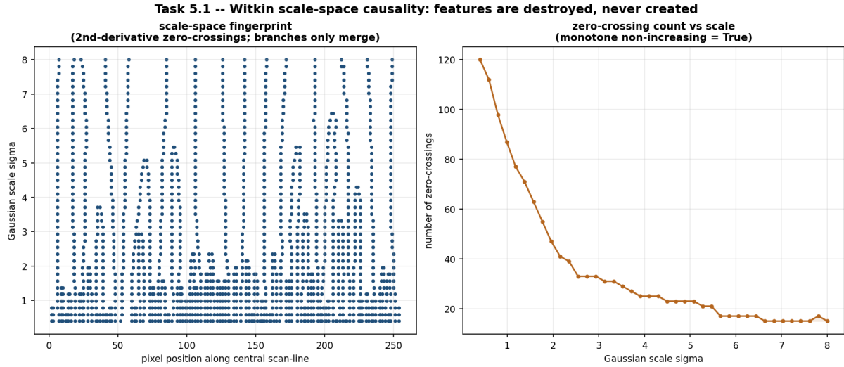
Figure 6: Left: zero-crossing fingerprint (branches only merge upward). Right: zero-crossing count is monotone non-increasing in \sigma .
