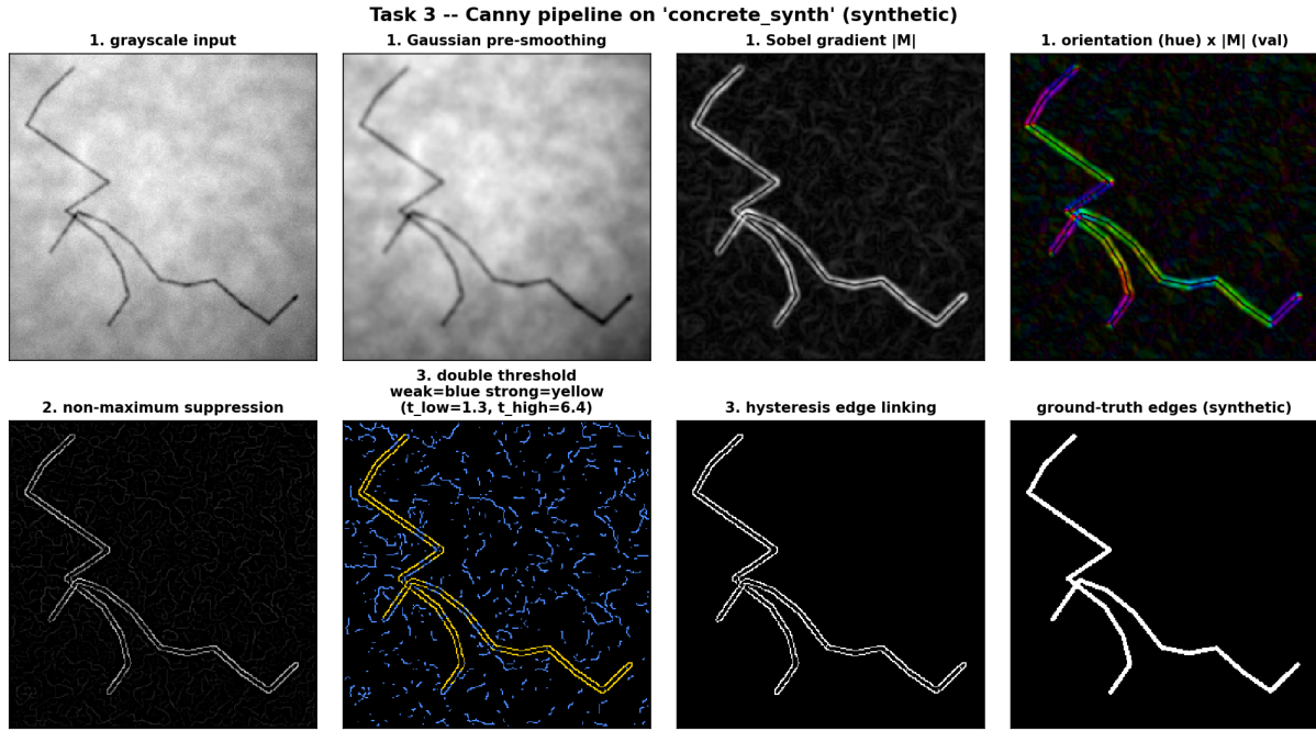
Figure 1: Four-stage Canny on a concrete-crack sample: grayscale, Gaussian pre-smoothing, Sobel |M| , orientation (hue) \times|M| (value), NMS, double-threshold classes (weak = blue, strong = yellow), hysteresis, ground truth.
