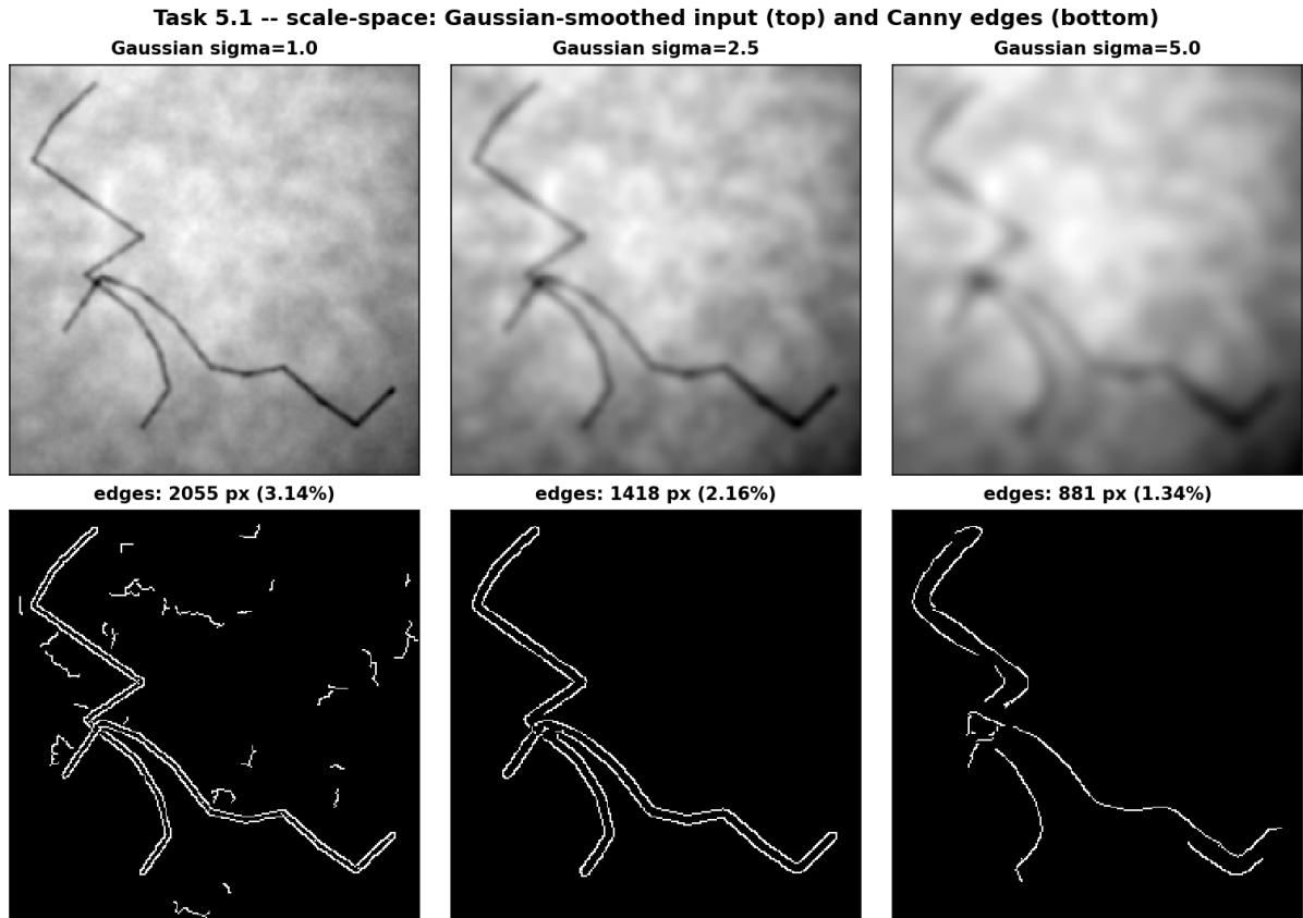
Figure 5: Scale-space: increasing \sigma destroys texture edges; the crack edges shift and merge but no new edges appear. Edge counts 2055 \rightarrow 1418 \rightarrow 881 .
