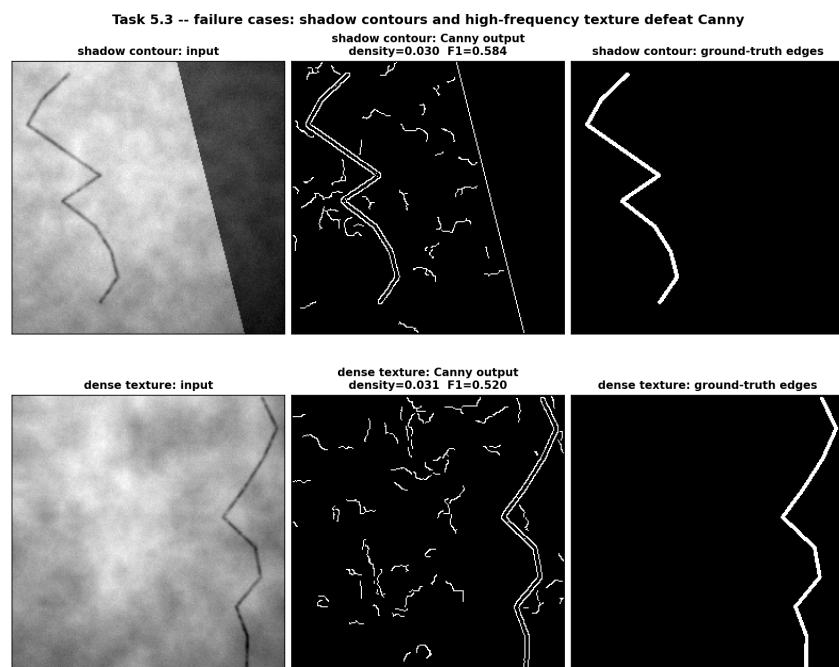
Figure 8: Failure cases. Row 1: a cast-shadow contour becomes a strong false edge. Row 2: dense texture yields a fragmented map that buries the crack. Columns: input, Canny output, ground truth.
