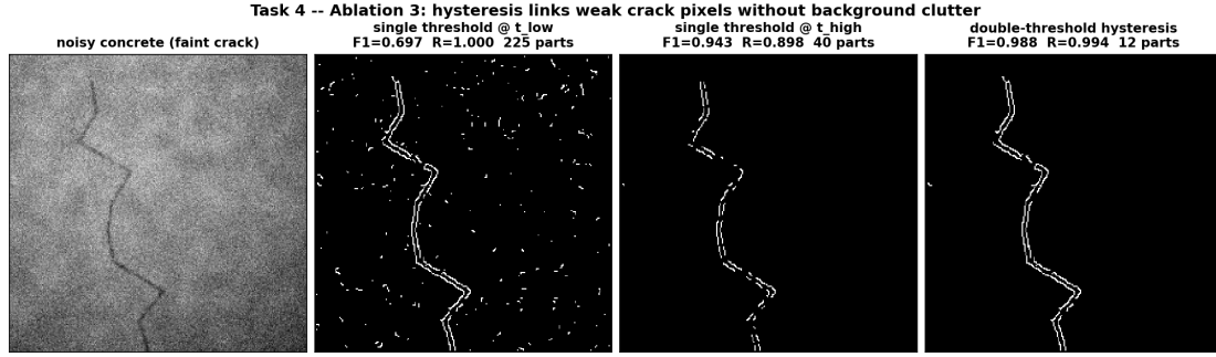
Figure 4: Ablation 3. Left to right: noisy input; single threshold at T_{\text{low}} ; single threshold at T_{\text{high}} ; double-threshold hysteresis.
