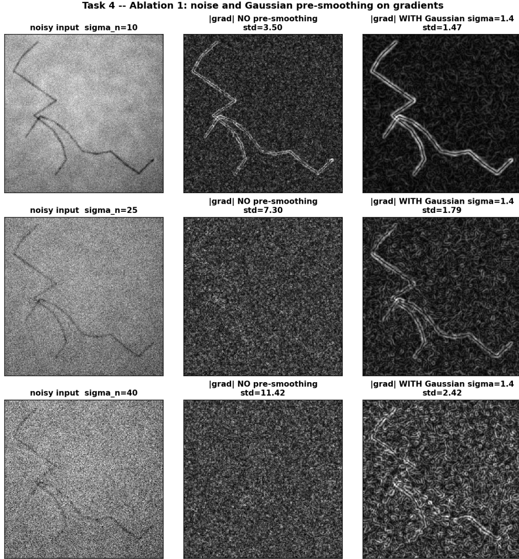
Figure 2: Ablation 1. Rows: \sigma_n \in \{10, 25, 40\} . Columns: noisy input; |\nabla| without pre-smoothing; |\nabla| with Gaussian pre-smoothing.
