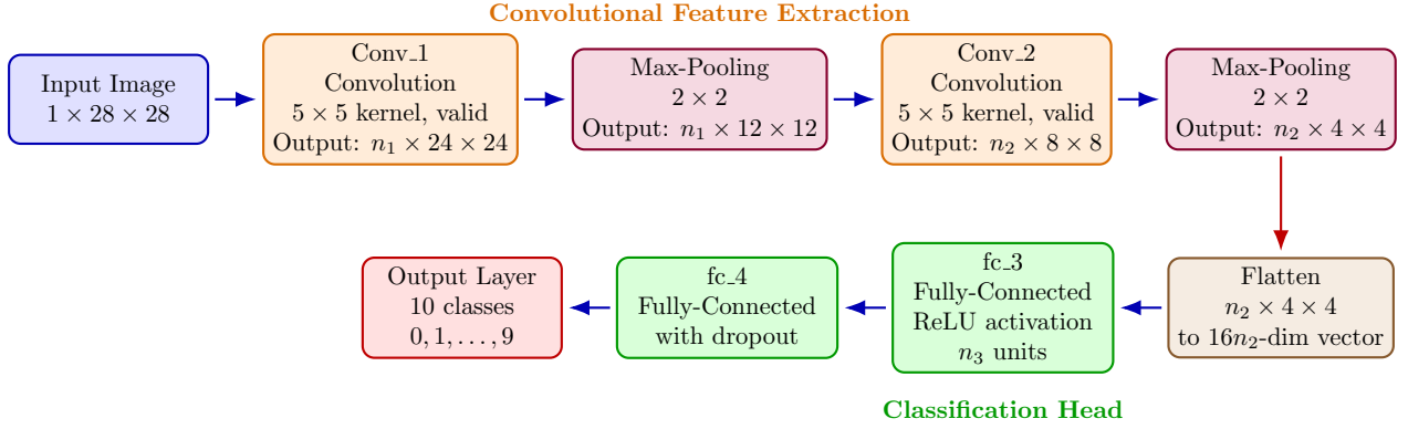
Figure 9.2: Flow diagram of a basic CNN architecture in PyTorch tensor order. The model takes an input tensor of size 1 \times 28 \times 28 , applies two convolutional layers with 5 \times 5 valid kernels and 2 \times 2 max-pooling, then flattens the resulting feature maps and passes them through fully connected layers for classification.
