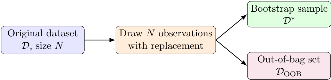
Figure 8.4: Bootstrap sampling creates a resampled training set and an associated out-of-bag set.
