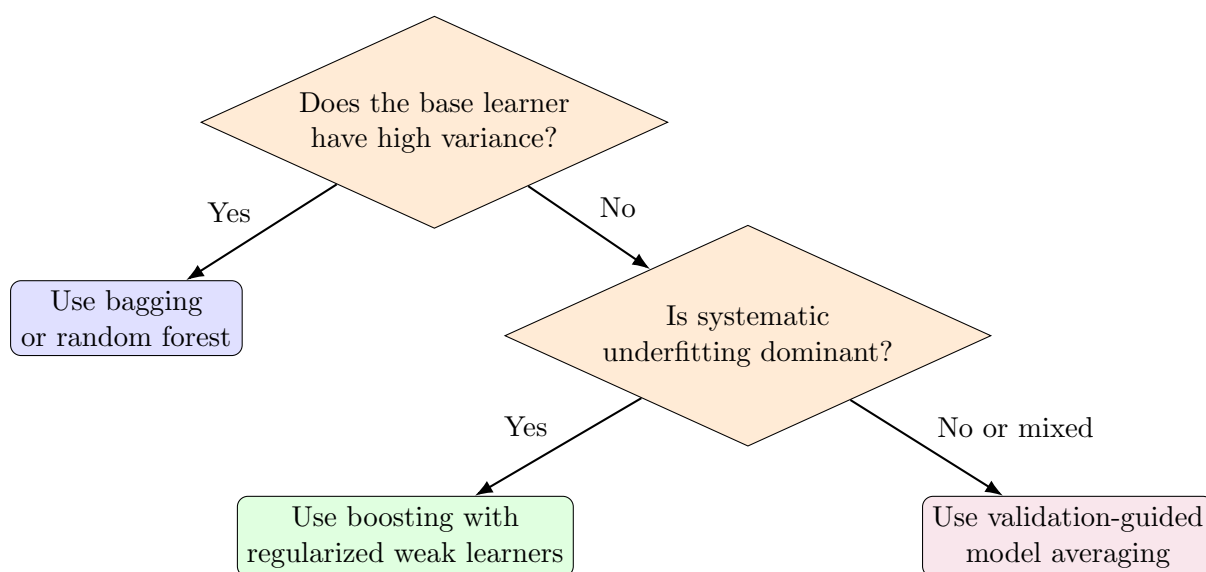
Figure 8.7: Simplified selection guide for bagging, boosting, and general model averaging.
