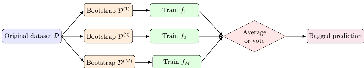
Figure 8.5: Bagging trains independent members on bootstrap resamples and combines their predictions in parallel.
