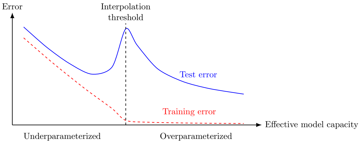
Figure 8.3: Conceptual double-descent curve. Test error may peak near the interpolation threshold and decrease again in the overparameterized regime.
