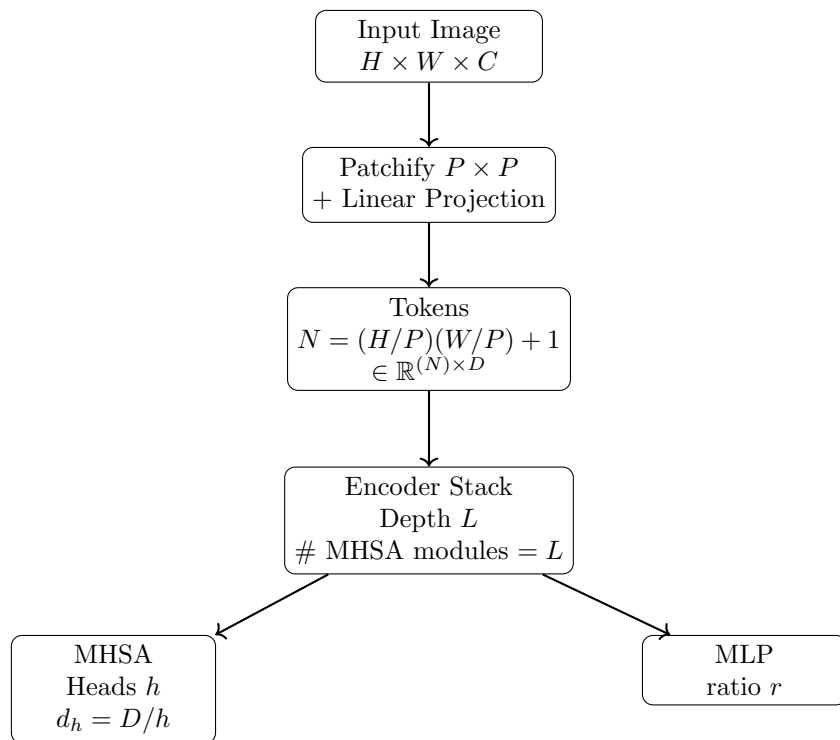
Figure 11.5: Tree-style view of ViT. The encoder stack has depth L ; each layer contains one MHA (therefore total attention modules = L ) with h heads and an MLP block.
