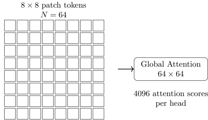
Figure 11.2: Small ViT attention example. A 16 \times 16 image with 2 \times 2 patches produces an 8 \times 8 token grid. Since ViT uses global self-attention, the attention matrix has size 64 \times 64 .
