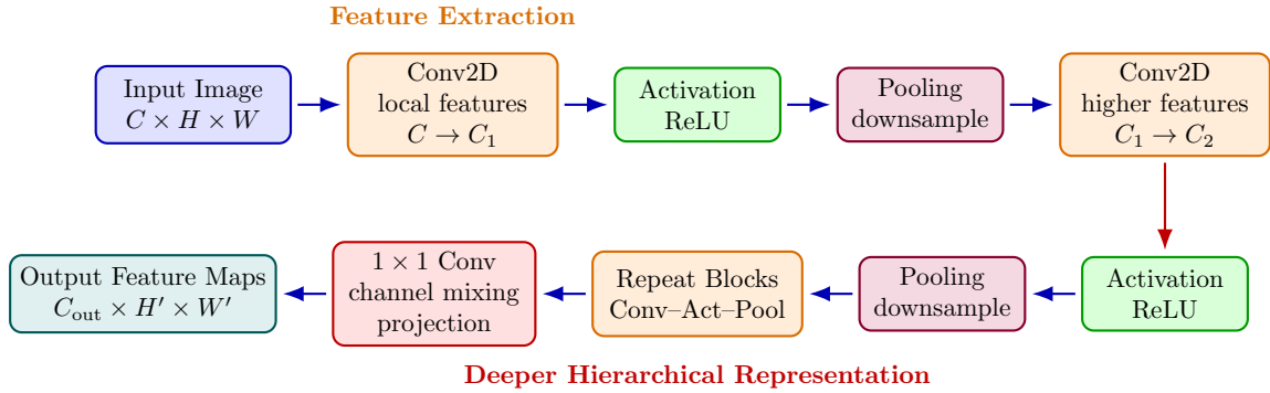
Figure 9.1: Basic CNN flow diagram in PyTorch tensor order. A CNN applies convolution, activation, and pooling repeatedly to learn hierarchical feature maps. A 1 \times 1 convolution can mix channels and change the number of output feature maps without changing the spatial resolution.
