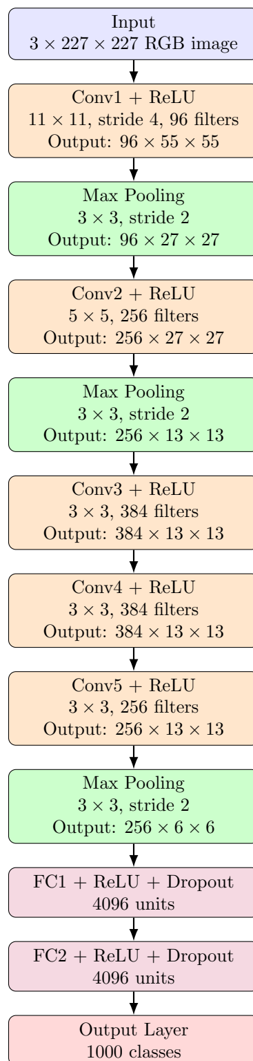
Figure 9.5: A simple flow diagram of the AlexNet architecture.
