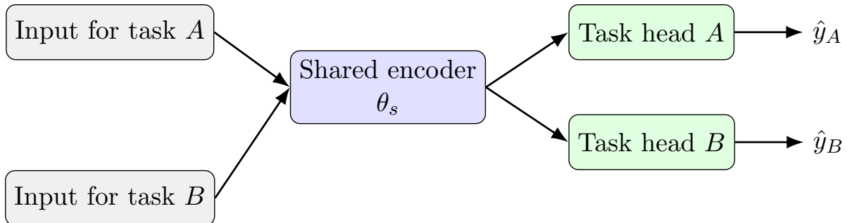
Figure 8.2: Hard parameter sharing in multi-task learning. The encoder parameters are exactly shared, while the output heads remain task-specific.
