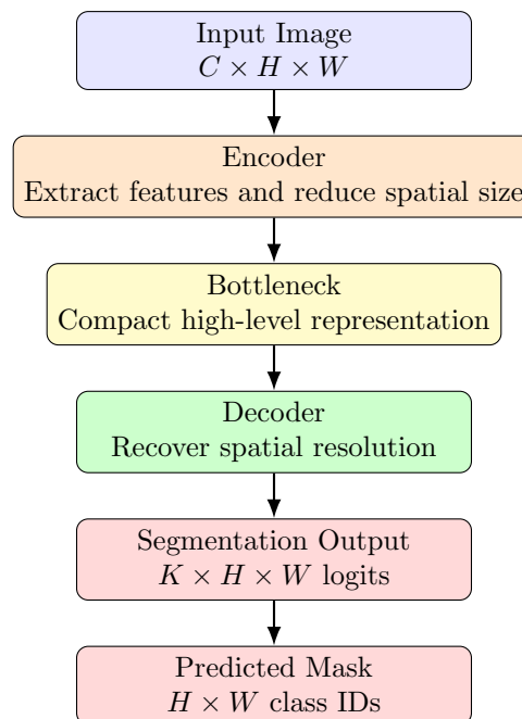
Figure 10.1: A simple encoder-decoder flow for image segmentation.
