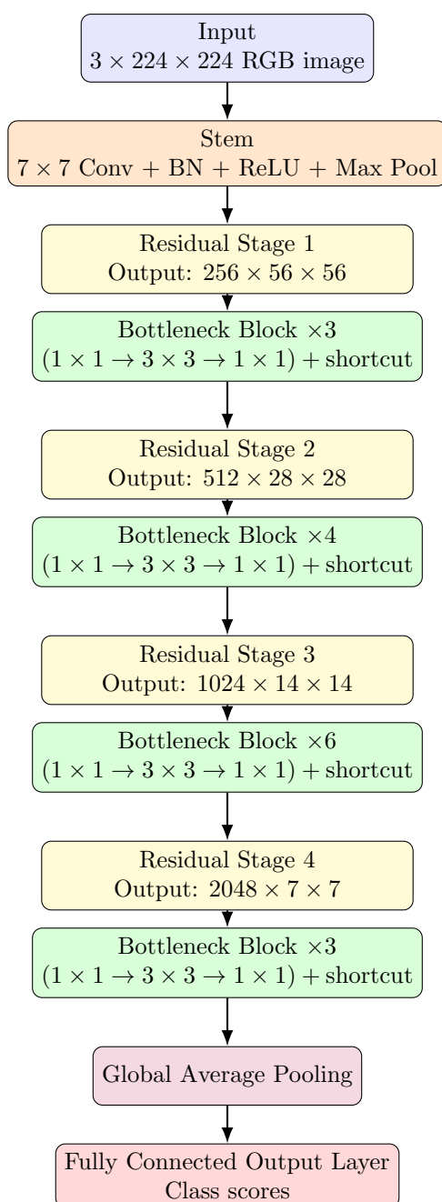
Figure 9.9: Repeating bottleneck blocks in a ResNet-50 style architecture. The four residual stages repeat bottleneck blocks 3, 4, 6, and 3 times.
