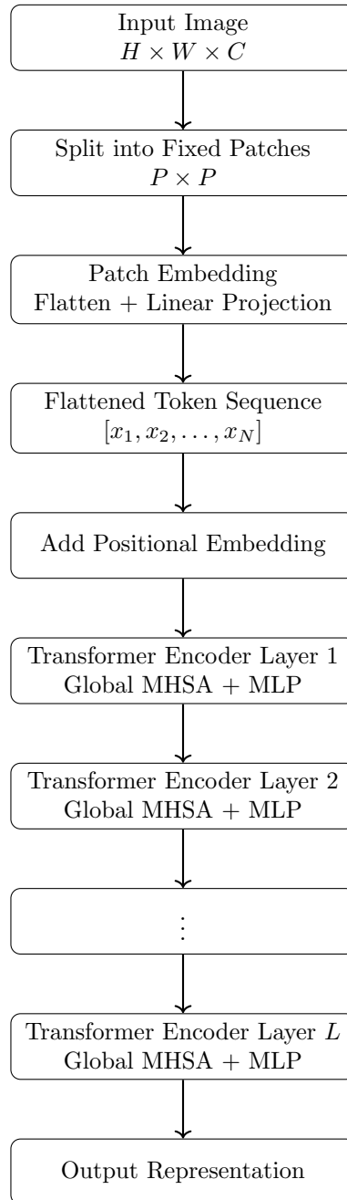
Figure 11.1: Architectural flow of the Vision Transformer. ViT converts the image into a flat sequence of patch tokens and applies global self-attention across all tokens in every encoder layer.
