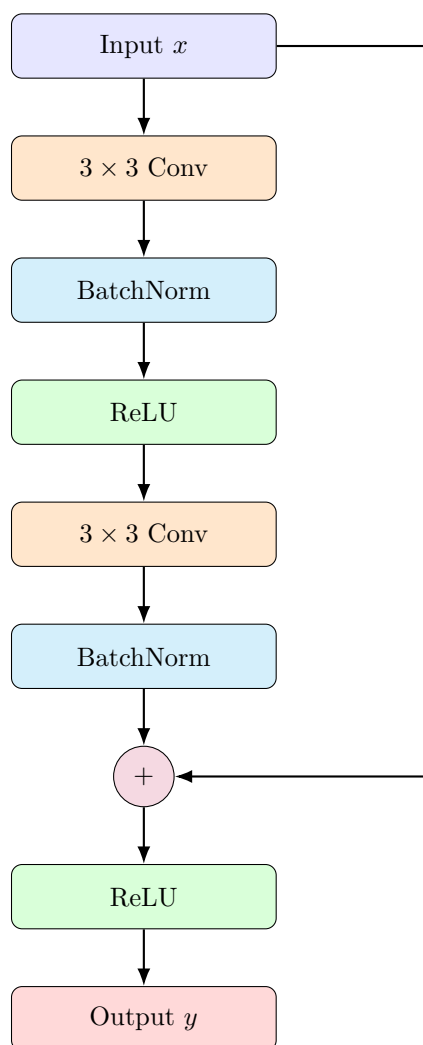
Figure 9.10: A basic ResNet residual block. The input x passes through convolution layers and also skips directly to the addition operation.
