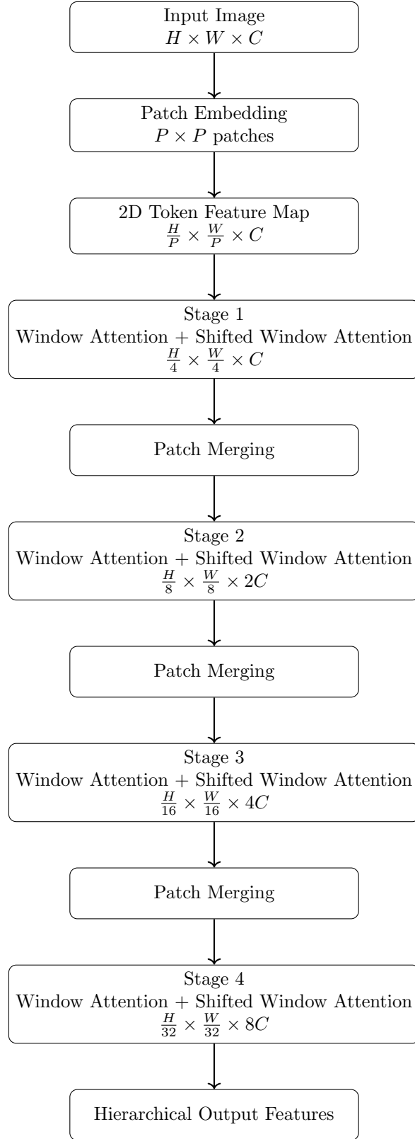
Figure 12.1: Architectural flow of the Swin Transformer. Swin keeps image tokens as a two-dimensional feature map, applies attention inside local windows, uses shifted windows for cross-window interaction, and builds a hierarchical feature representation through patch merging.
