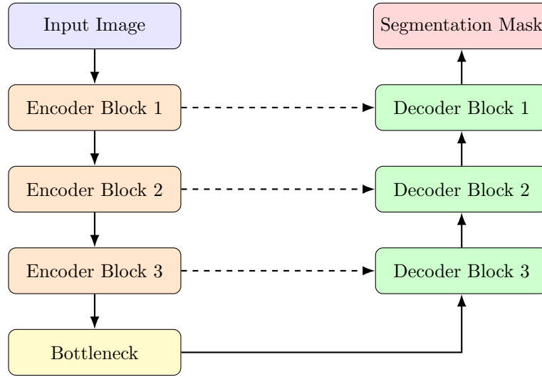
Figure 10.2: A simplified U-Net architecture. Dashed arrows represent skip connections from encoder blocks to decoder blocks.
