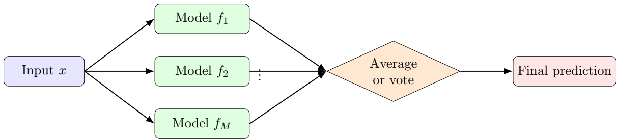
Figure 8.1: Parallel committee architecture. Each member processes the same input, and a combination rule produces the final prediction.
