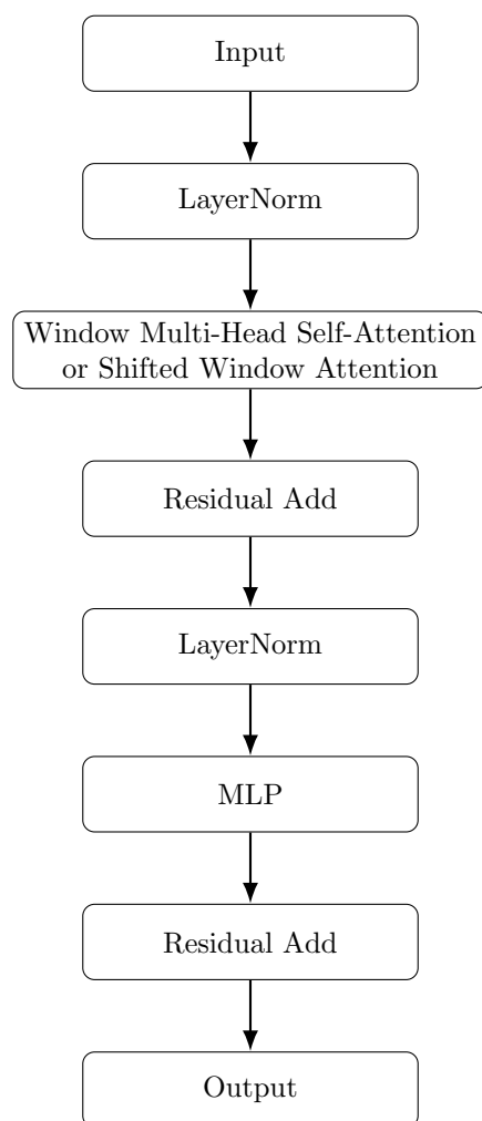
Figure 12.8: Internal flow of a Swin Transformer block.
