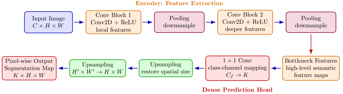
Figure 9.3: Basic FCN flow diagram for semantic segmentation in PyTorch tensor order. The encoder extracts hierarchical feature maps using convolution and pooling. A 1 \times 1 convolution maps the learned feature channels to K class-score channels, and upsampling restores the spatial resolution to produce a pixel-wise segmentation map.
