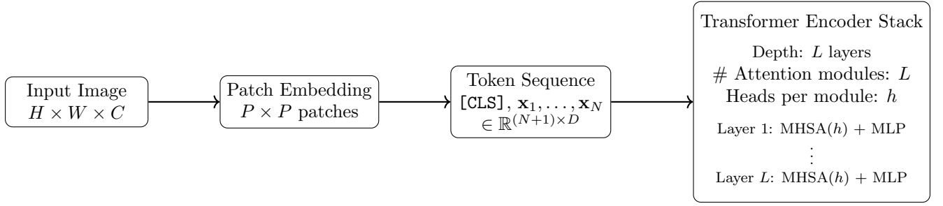
Figure 11.3: High-level architecture of the Vision Transformer (ViT). An input image is split into non-overlapping patches, embedded into a token sequence, and processed by a Transformer encoder stack of depth L . Each encoder layer contains exactly one multi-head self-attention (MHSA) module (so the number of attention modules is L ), and each MHSA uses h attention heads.
