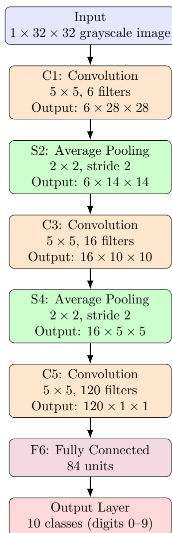
Figure 9.4: A simple flow diagram of the LeNet-5 architecture.
