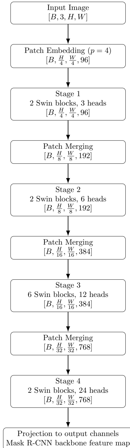
Figure 12.9: Example Swin Transformer backbone configuration with embed\_dim = 96 , depths = (2, 2, 6, 2) , and num\_heads = (3, 6, 12, 24) .
