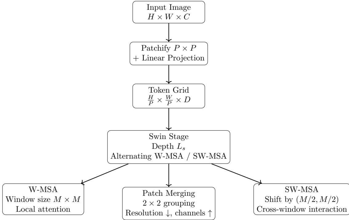
Figure 12.4: Tree-style view of one Swin Transformer stage. Each stage contains L_s Swin blocks with alternating regular window attention (W-MSA) and shifted-window attention (SW-MSA). Patch merging connects one stage to the next by reducing spatial resolution and increasing feature dimension.
