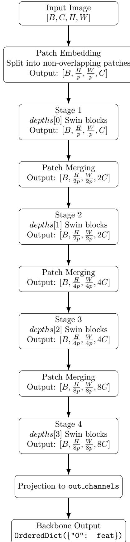
Figure 12.6: Overall flow of a Swin Transformer backbone. Here, p denotes patch size and C denotes the base embedding dimension.
