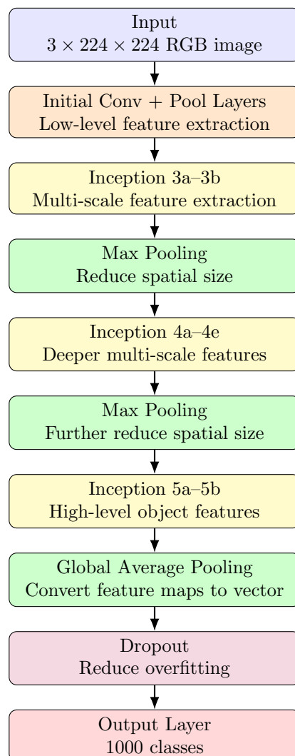
Figure 9.8: A simple flow diagram of the GoogLeNet architecture.
