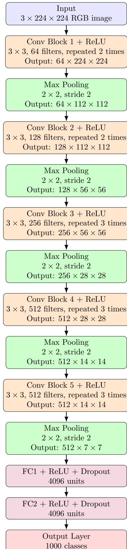
Figure 9.6: A simple flow diagram of the VGG16 architecture.
