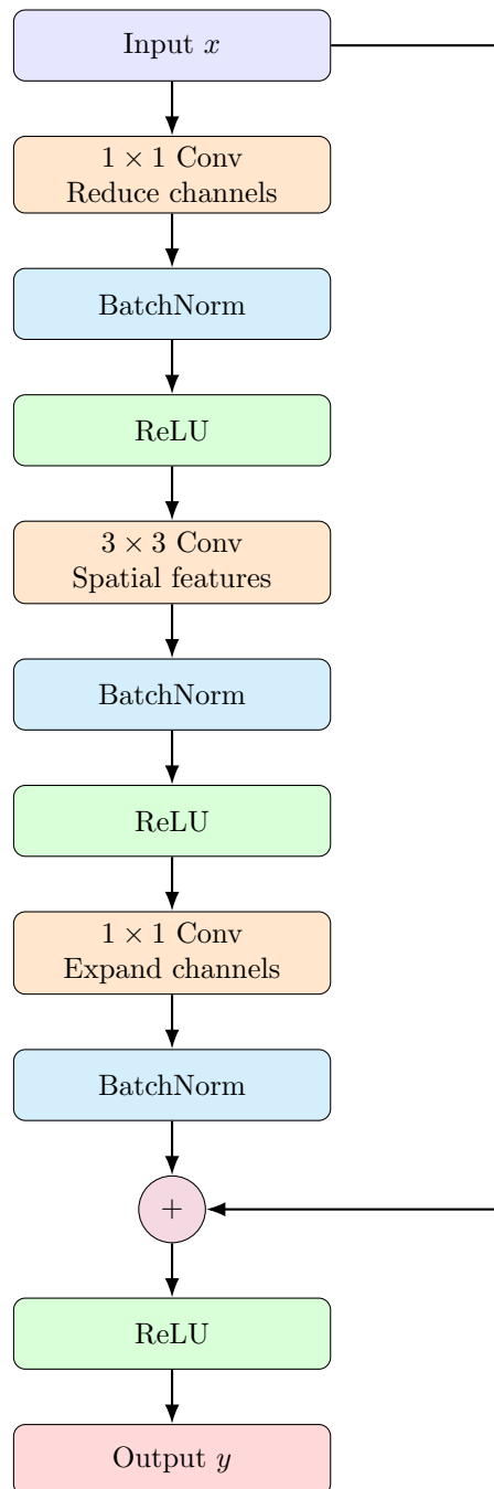
Figure 9.11: A bottleneck ResNet block. The 1 \times 1 convolutions reduce and then expand the channel dimension, while the 3 \times 3 convolution extracts spatial features.
