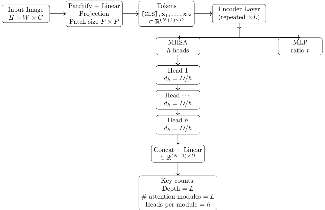
Figure 11.4: Hydra/tree-style view of ViT without overflow. Tokens pass through an encoder layer repeated \times L . Each layer contains exactly one MHSA (so the number of attention modules is L ) with h heads and one MLP block. The MHSA splits into h heads and merges back via concatenation to dimension D .
