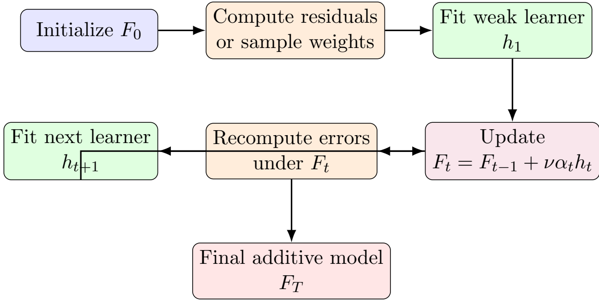
Figure 8.6: Boosting is sequential. Each new weak learner is trained using information from the current ensemble error.
