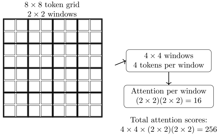
Figure 12.2: Small Swin Transformer attention example. A 16 \times 16 image with 2 \times 2 patches produces an 8 \times 8 token grid. With a 2 \times 2 window size, the grid contains 4 \times 4 windows, and attention is computed locally inside each window.
