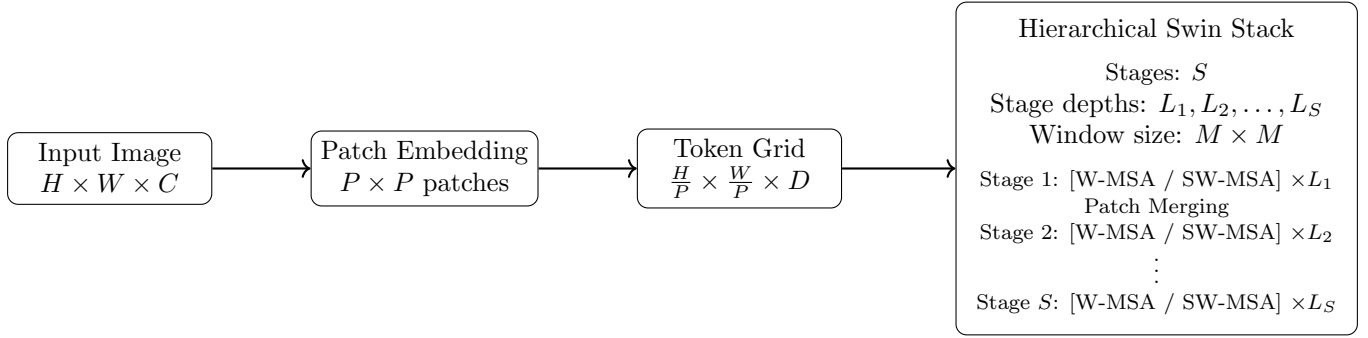
Figure 12.3: High-level architecture of the Swin Transformer. An input image is partitioned into patches and embedded into a 2D token grid. The token grid is processed by a hierarchical sequence of stages. Within each stage, Swin blocks alternate between regular window attention (W-MSA) and shifted-window attention (SW-MSA). Patch merging layers between stages reduce spatial resolution and increase channel dimension.
