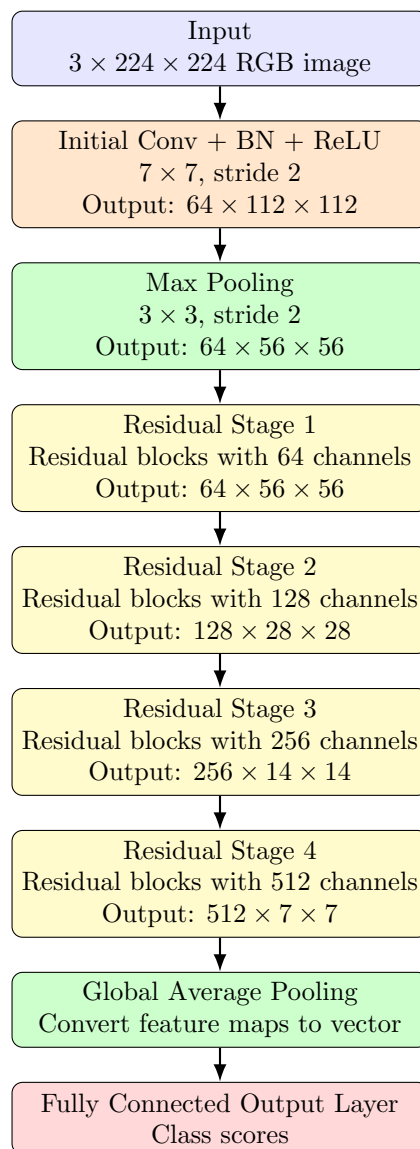
Figure 9.12: A simple flow diagram of a standard ResNet architecture.
