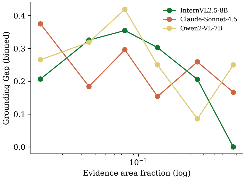
GG vs evidence-region size
