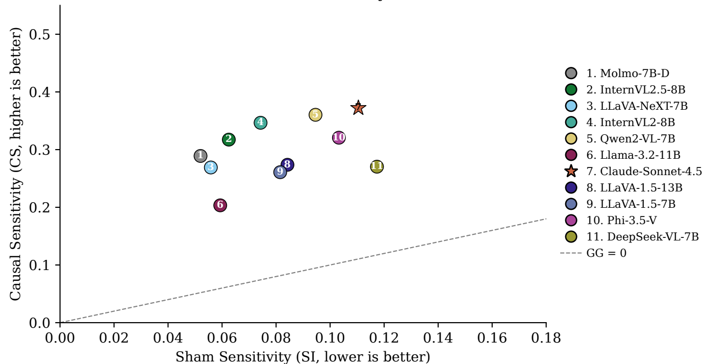
Causal vs Sham sensitivity (blur)
