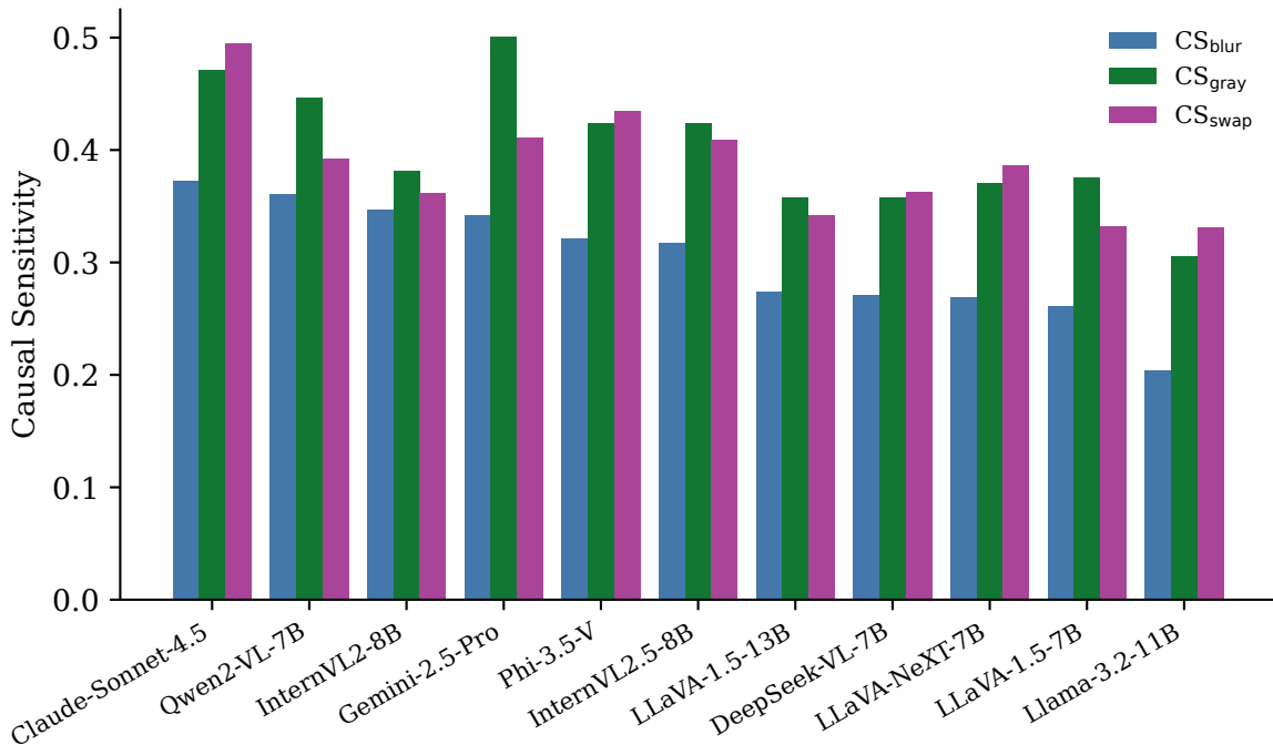
CS by intervention operator
