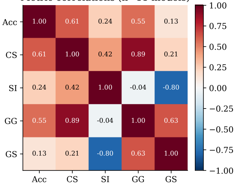
Metric correlations (n=11 models)
