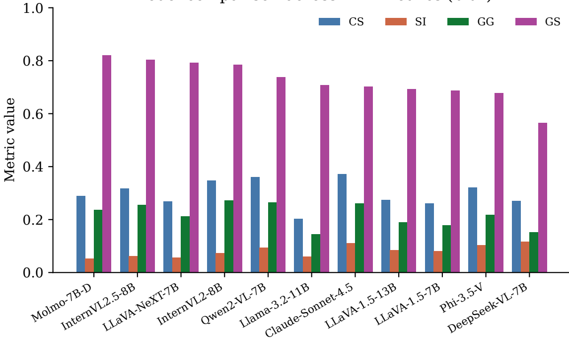
Model comparison across MEI metrics (blur)
