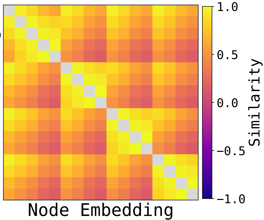
Node Embedding
