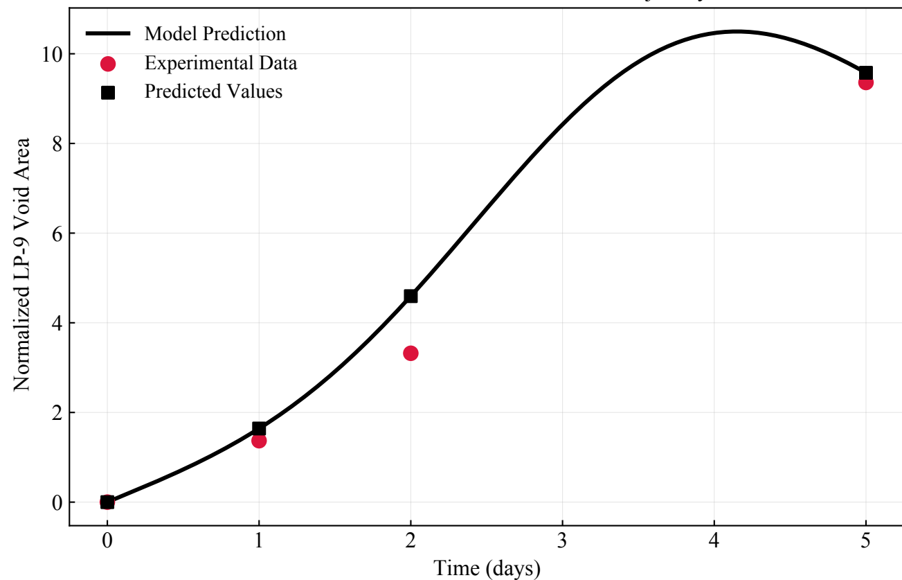
OVCAR3: Predicted Tumor+MSC+M2 trajectory
