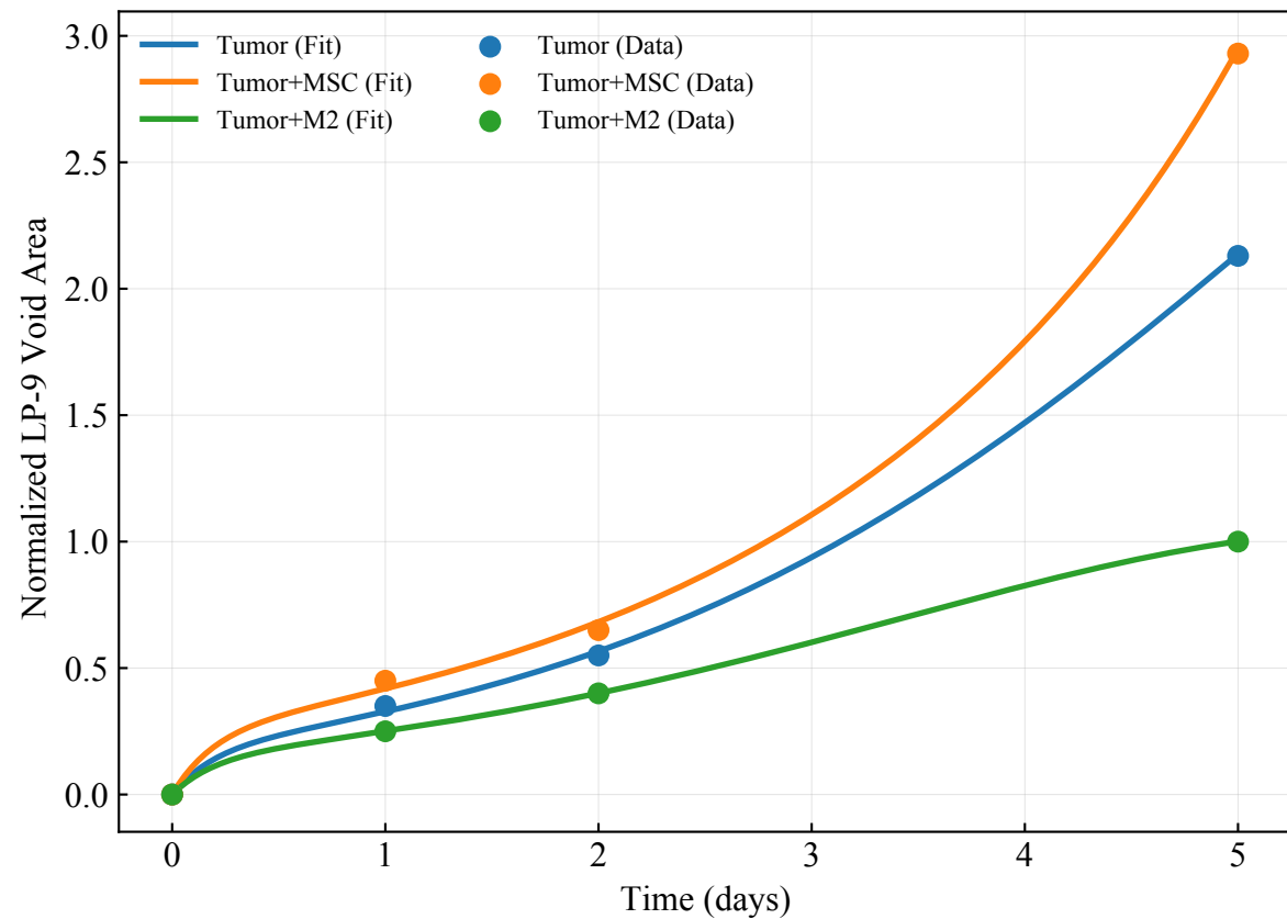
OVCAR4: Calibration
