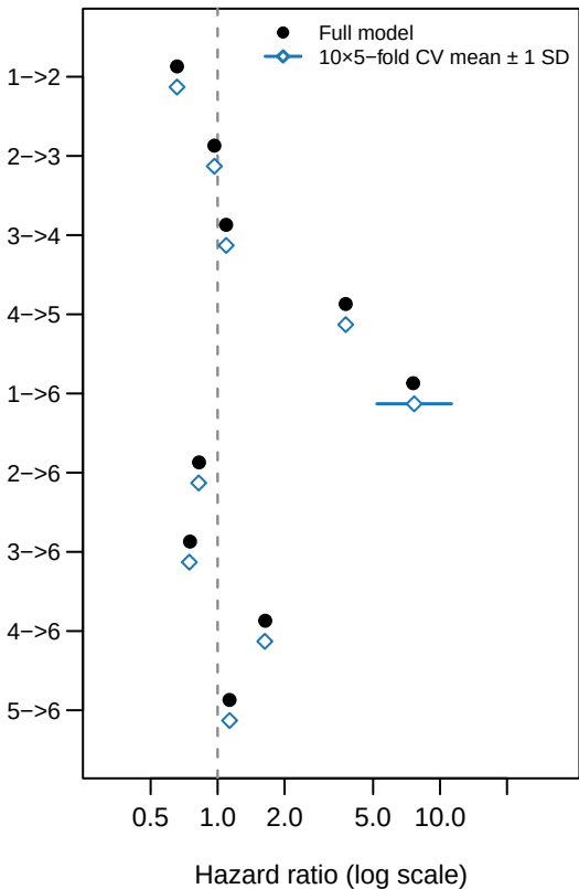
(b) Hypertension (HTN vs. no HTN)
