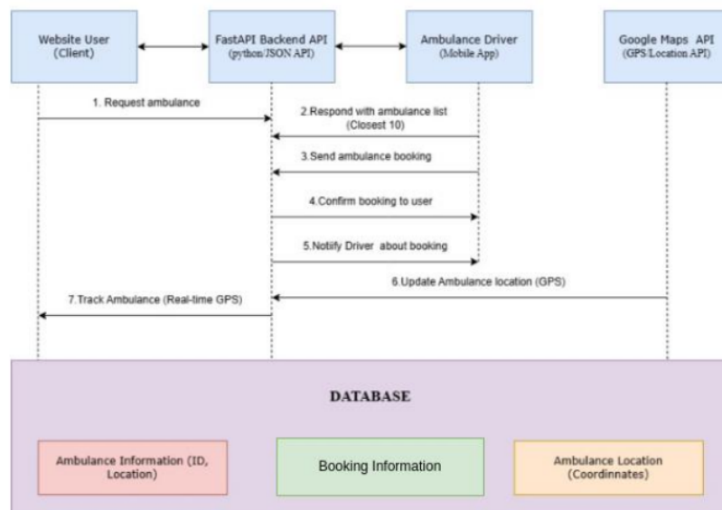
Figure 1 System Architecture
