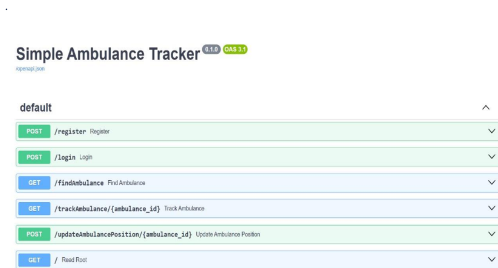
Figure 4. FastAPI-Based backend
