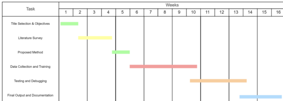
Figure 7. Gantt Chart
