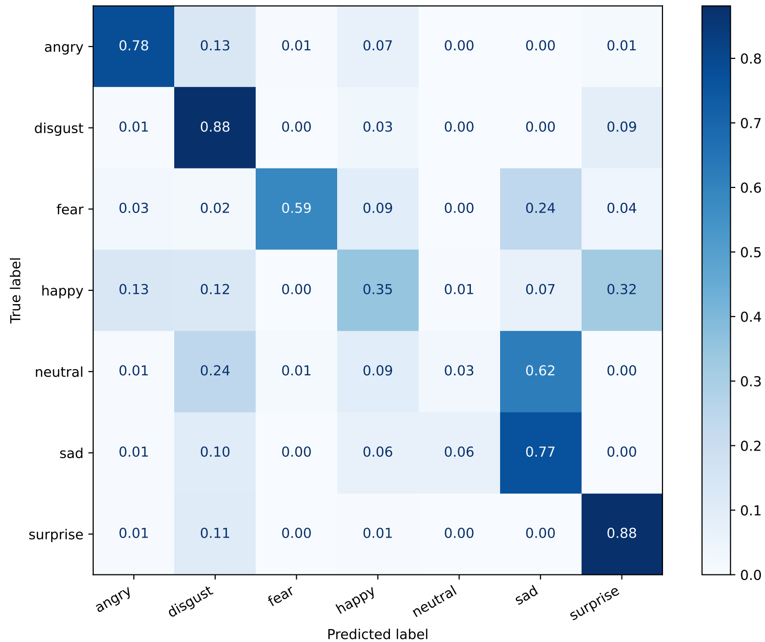
HuBERT + DPPMI — Normalized Confusion Matrix
