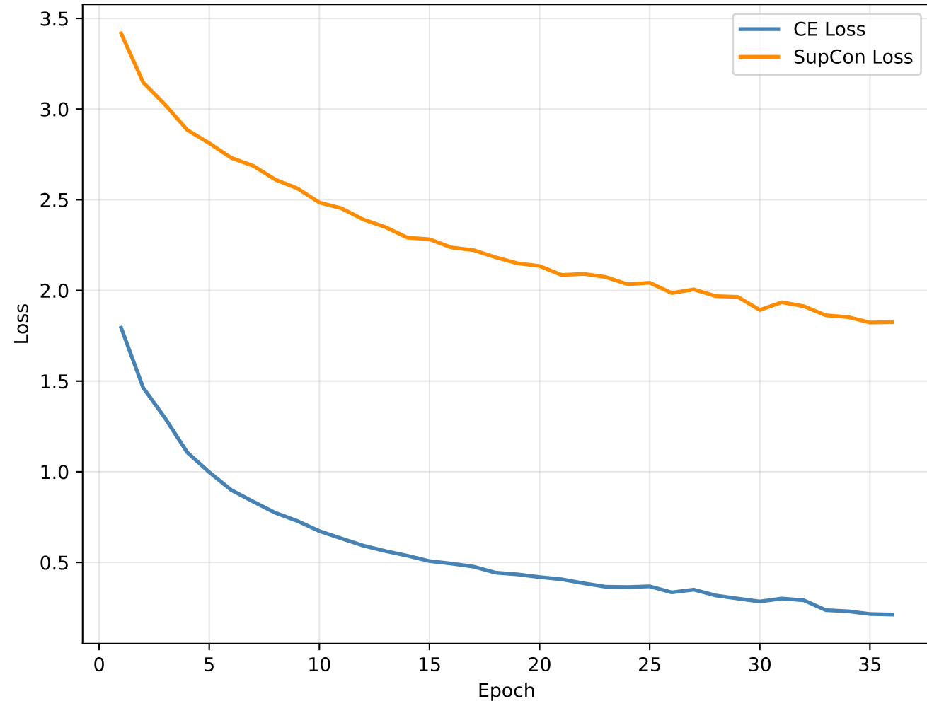
Loss Curves
