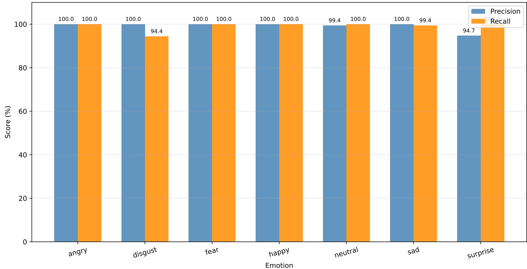
HuBERT + DPPMI + SupCon — Per-Emotion Precision vs Recall
