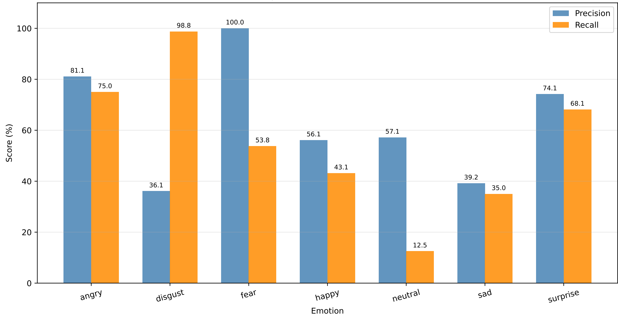
HuBERT Only — Per-Emotion Precision vs Recall
