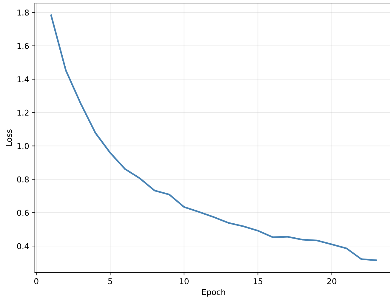
Loss Curves
