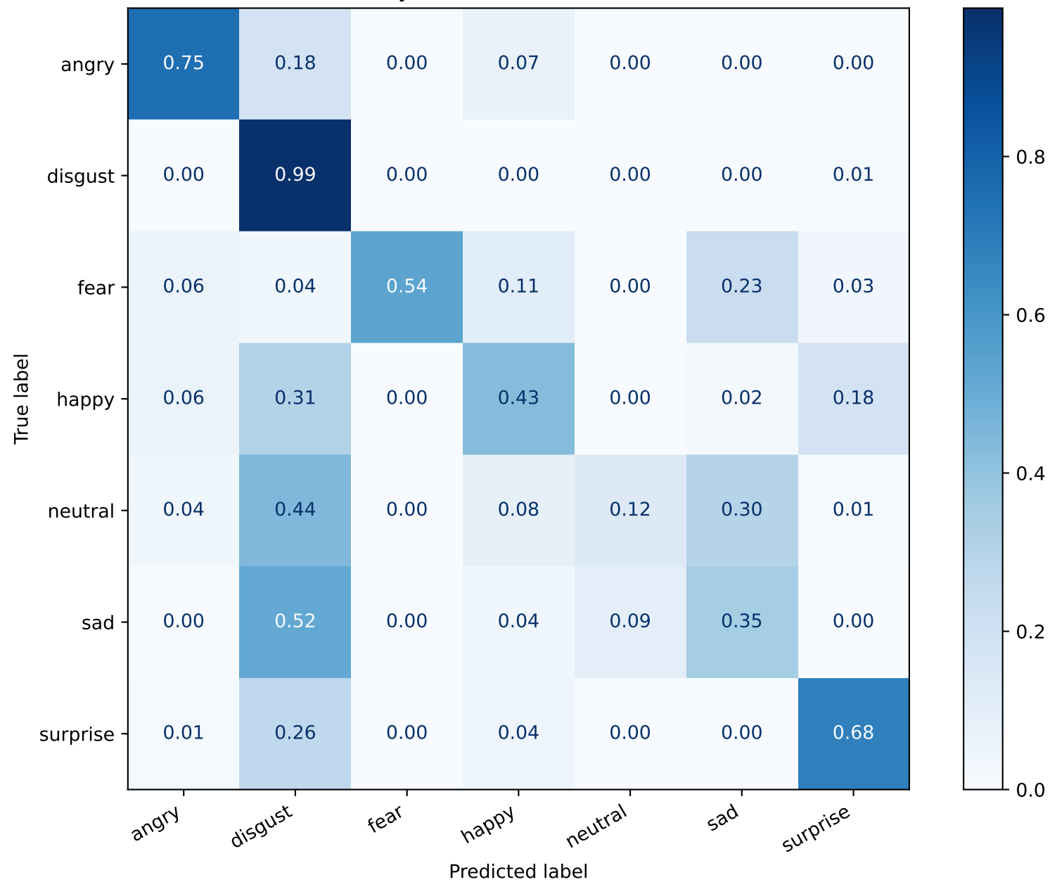
HuBERT Only — Normalized Confusion Matrix
