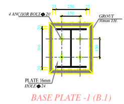
BASE PLATE PLAN
