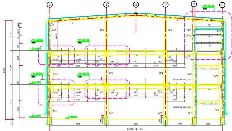
FRAME FROM AX. 2 SCALE 1:100
