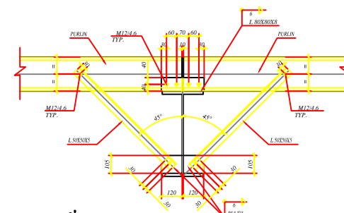
* TYP. DETAIL OF KNEE BRACING WITH PURLINS SCALE 1:30
