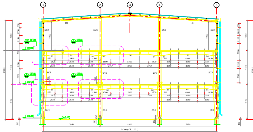
FRAME FROM AX. 3 TO 10 SCALE 1:100
