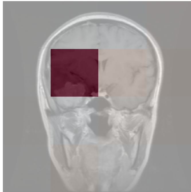
MCaI Calibrated LIME Pred: [0.00, 1.00, 0.00, 0.00]
