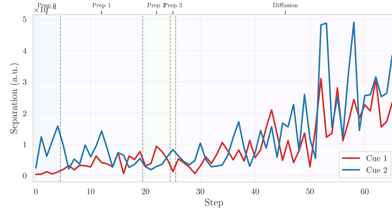
Centroid separation
