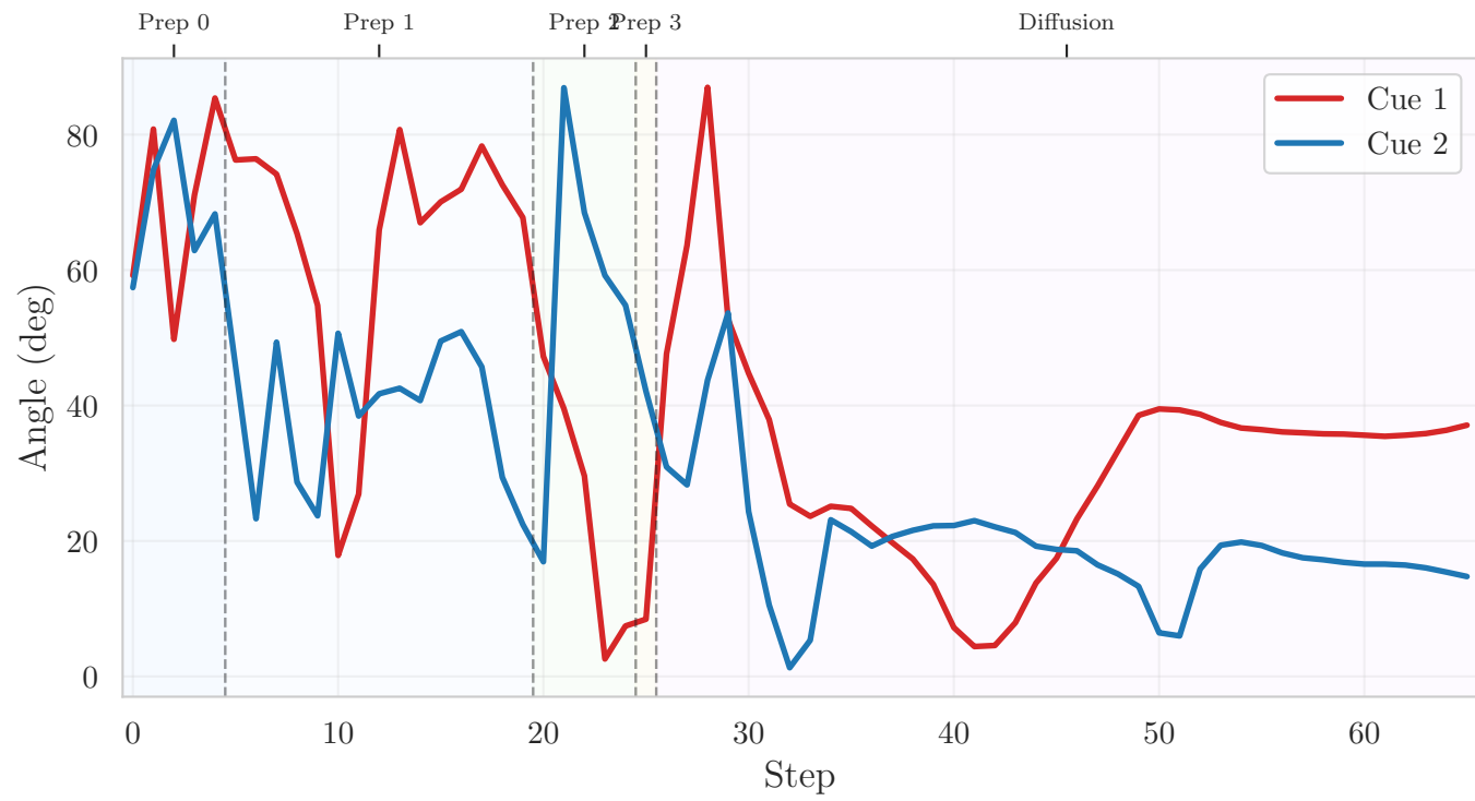
Centroid separation
