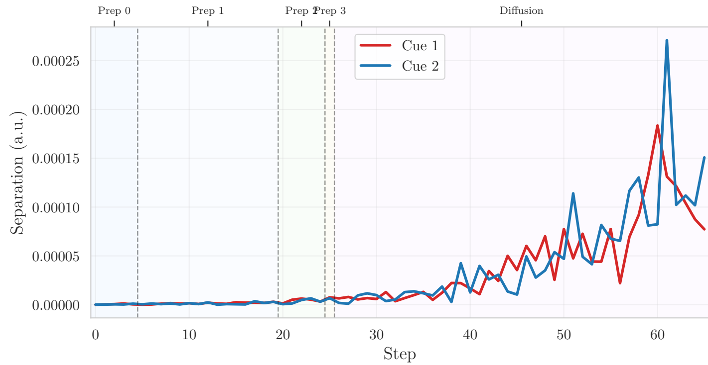
Centroid separation
