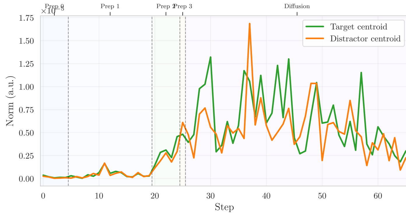
Centroid norm
