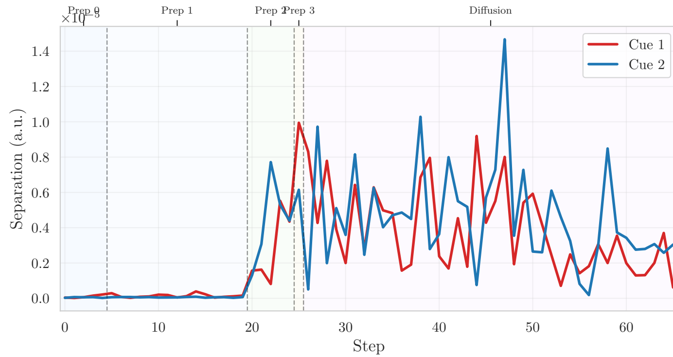
Centroid separation
