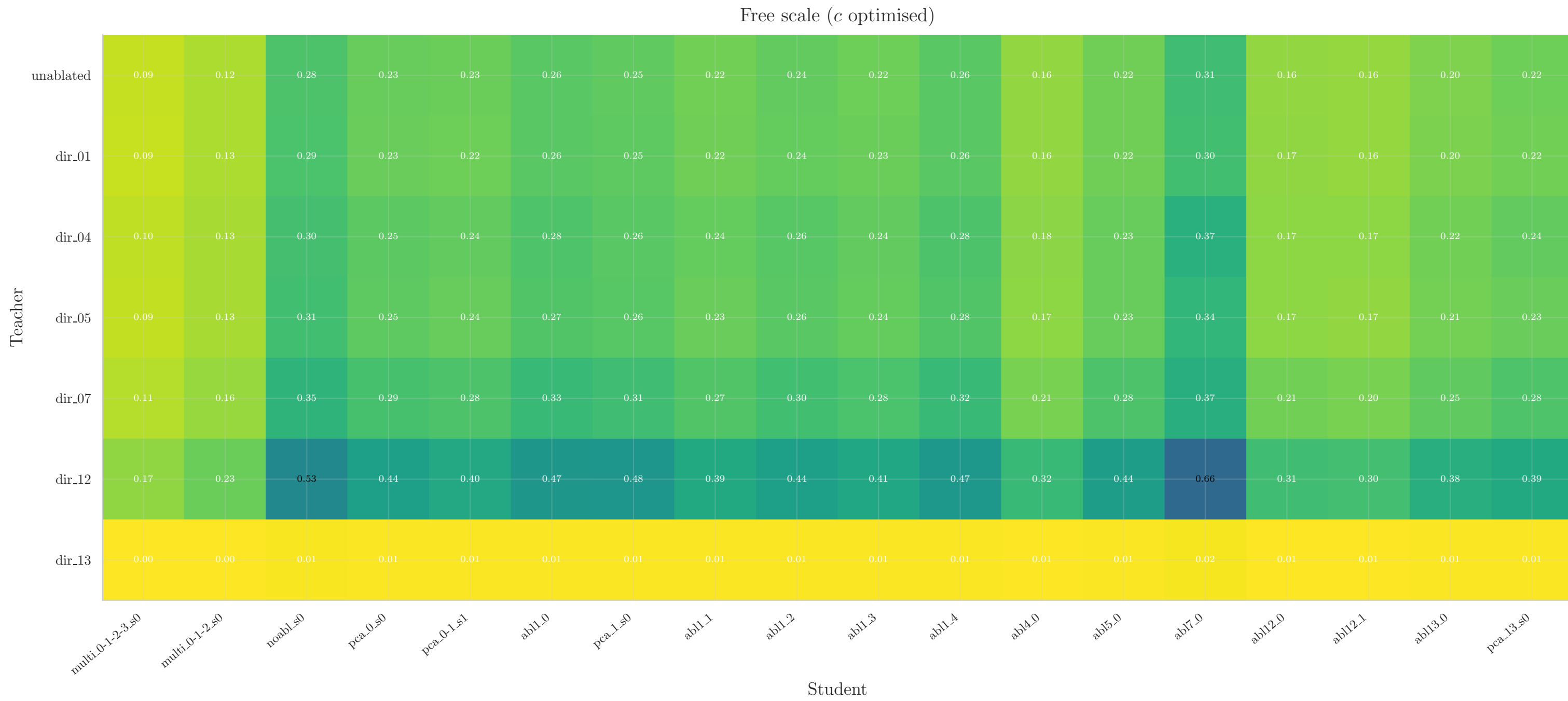
Procrustes residual: scaling comparison
