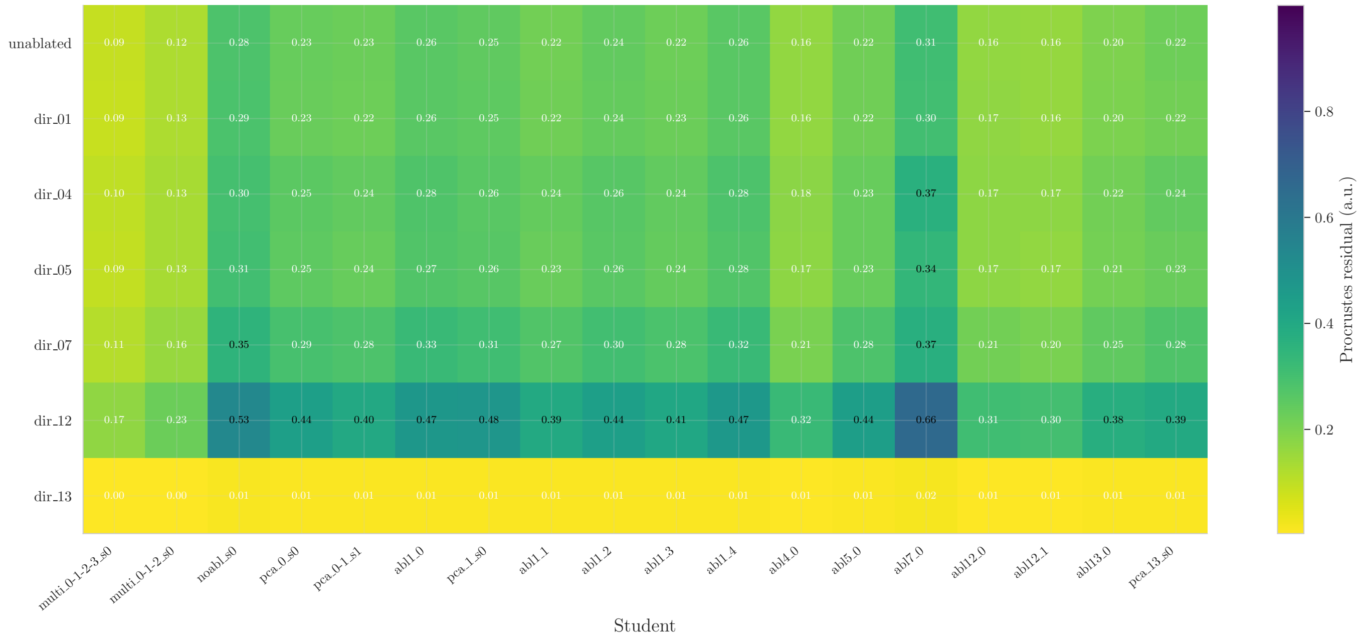
Procrustes residual (free scale)
