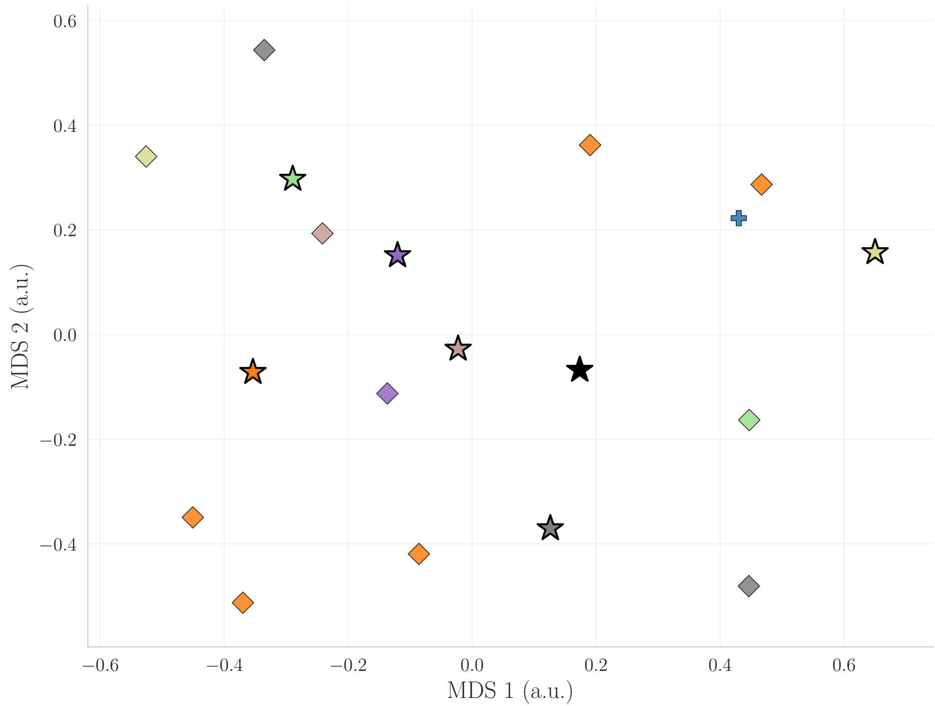
Procrustes MDS (non-metric)
