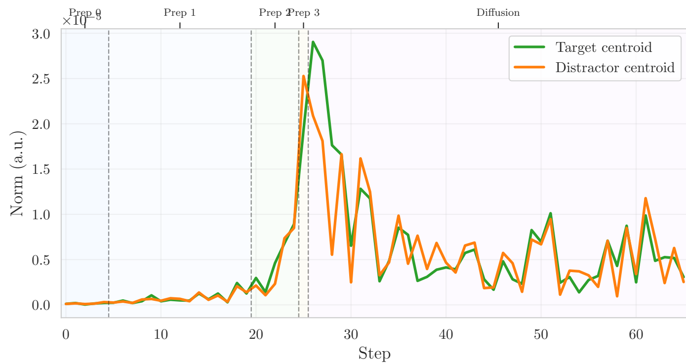
Centroid norm
